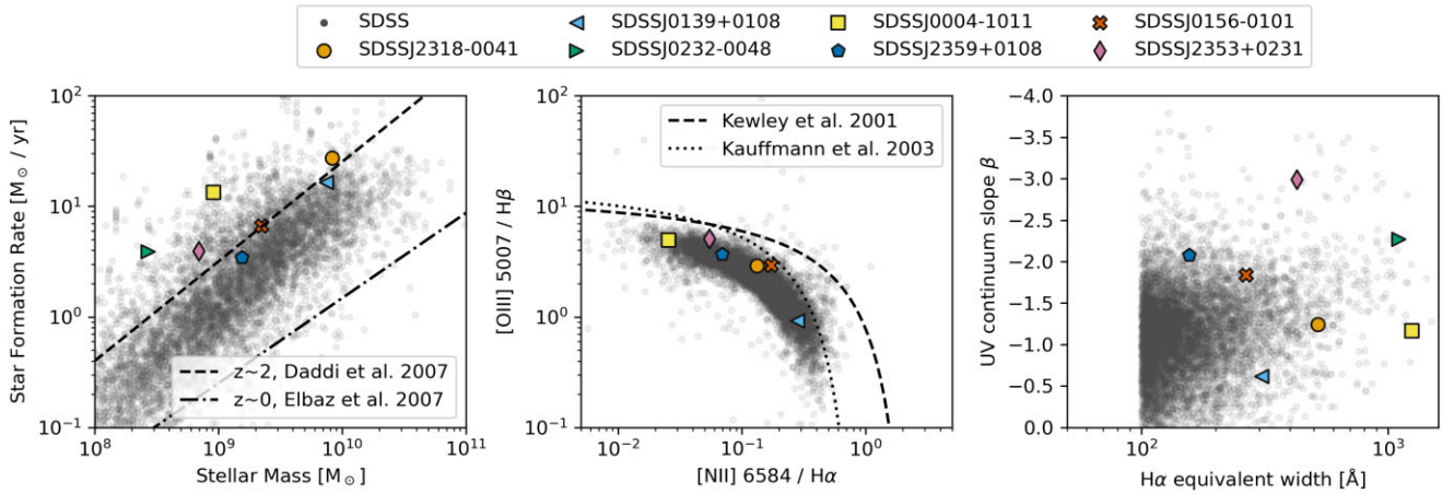
Figure 2. Sample selection figures. The left-hand panel shows star formation rate against stellar mass. The black points show a sample of 7000 SDSS galaxies with the single selection criterion of having a high ( \geq 100 \text{ \AA} ) H\alpha equivalent width. The dash-dotted line shows the star-forming main sequence relation at redshift \sim 0 derived from the SDSS from Elbaz et al. (2007) and the dashed line shows the main sequence at redshift 2 from Daddi et al. (2007). The central panel shows the BPT diagram (Baldwin, Phillips & Terlevich 1981) with the relations from Kewley et al. (2001) and Kauffmann et al. (2003) showing the demarcation between star forming galaxies and AGN. The third panel shows the UV slope \beta (assuming the standard proportionality f_\lambda \propto \lambda^\beta ) derived from GALEX photometry against the H\alpha equivalent width.
