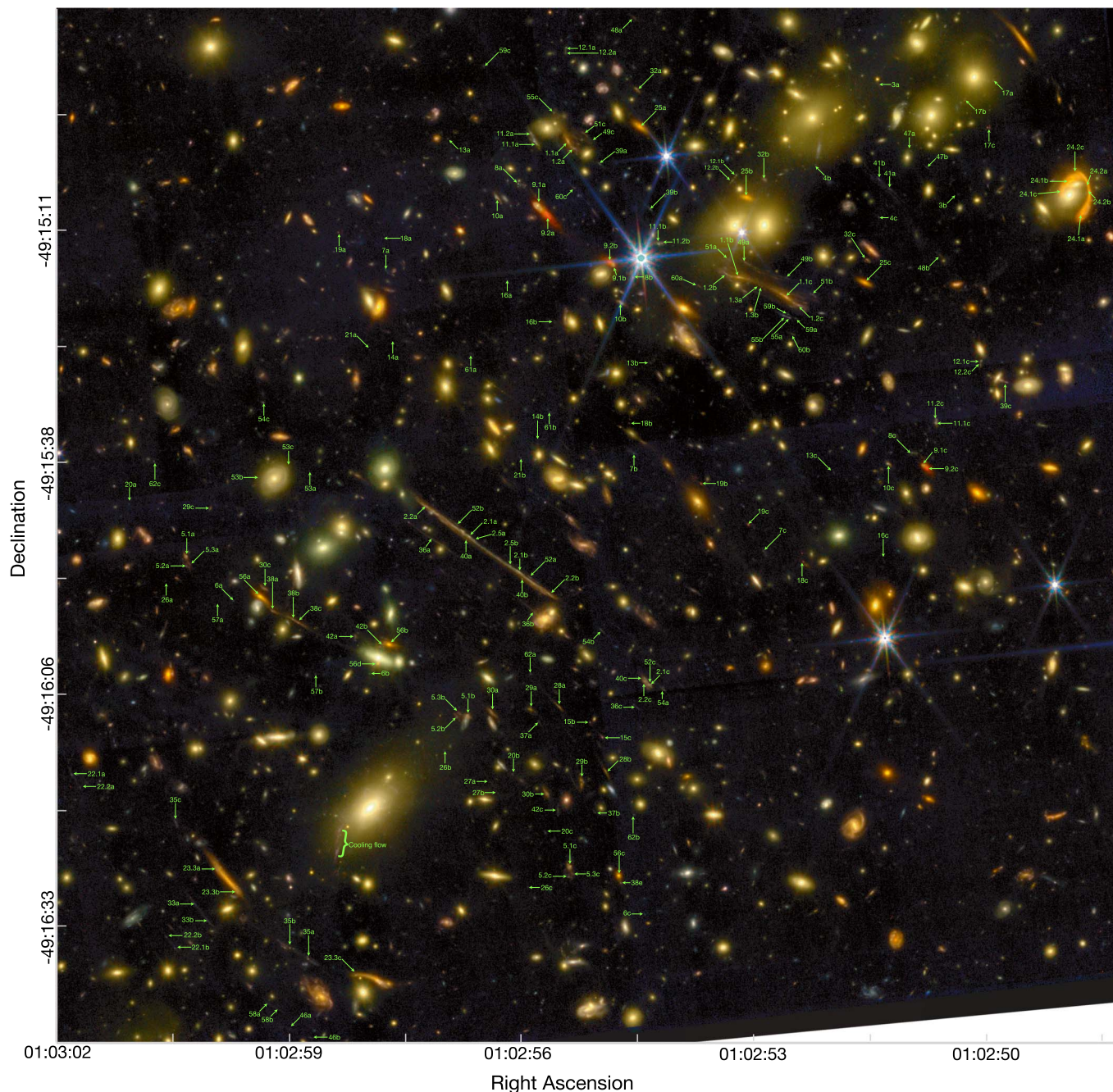
Figure 2. NIRCam color image of the central region of El Gordo. The image is 2\frac{1}{2} \times 2\frac{1}{2} on a side, and the orientation is North up and East to the left. The colors follow the prescription in TrilogY (Coe et al. 2012), with red showing F410M+F444W, green showing F200W+F277W+F356W, and blue showing F090W + F115W. All colors are multiplied by the sum of all the wide NIRCam filters (F090W + F115W + F150W + F200W + F277W + F356W + F444W) to the 1/4 power. The 56 image systems used in our lens model are labeled in green, as is the cooling flow detected in HST imaging. The axes give the R.A. and decl. in J2000 coordinates.
