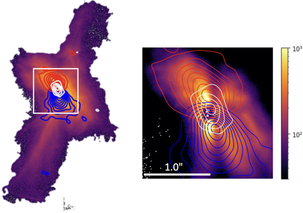
Fig. 7. Overlay of SPHERE (color scale) and ALMA (contours) data. On the left all the extended structure as seen with SPHERE, on the right a zoom-in of the innermost 2". White contours are ALMA 1.3 mm continuum, plotted at contours starting at, and increasing with, 3\sigma = 0.37 \text{ mJy beam}^{-1} . Red and blue contours are integrated ^{12}\text{CO} 2–1 emission over 10 \text{ km s}^{-1} blue- and red-shifted relative to the source velocity, taken as V_{\text{LSR}} = 4.5 \text{ km s}^{-1} . Red and blue contours are also drawn starting at (and increasing with) 3\sigma = 0.12 \text{ Jy beam}^{-1} \text{ km s}^{-1} . The ALMA data are aligned with the SPHERE data to have the stellar position at the center of the image; the continuum emission peaks \sim 0.06'' north of that position.
