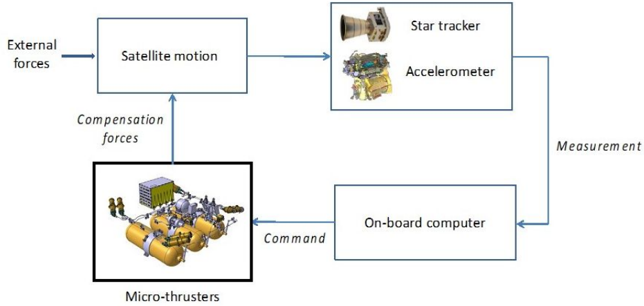
Fig. 3. Satellite Drag-Free and Attitude Control System
