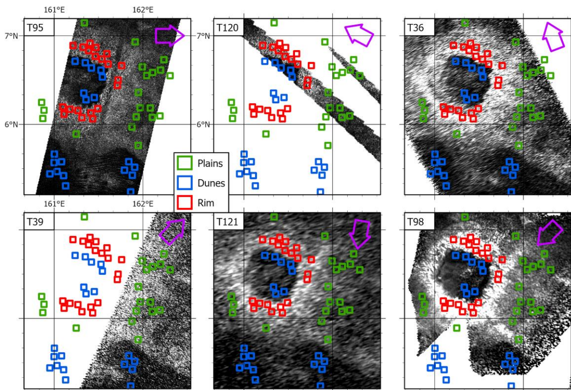
Figure 2: Radar data over Selk crater, corrected for incidence angle effects. The radar illumination direction is indicated by a magenta arrow. The backscatter properties are examined within three different regions: the crater rim, dunes, and plains/ejecta.
