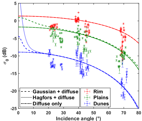
Figure 1: Backscatter curves for the three terrain units, with three different fits for each.
