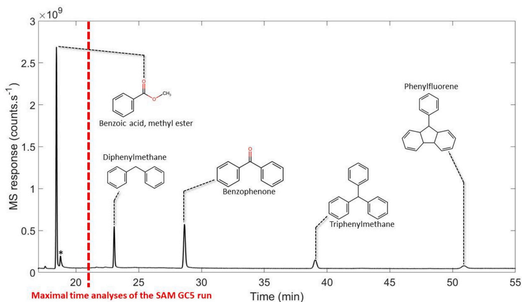
Fig. 11. Laboratory GC-MS analyses of the characteristic pyrolysis and derivatization products of organic salts in SAM GC5 conditions. The maximal time of analyses of the SAM GC5 run in situ is 21 min. (*) artifact of the column (stationary phase bleeding).
