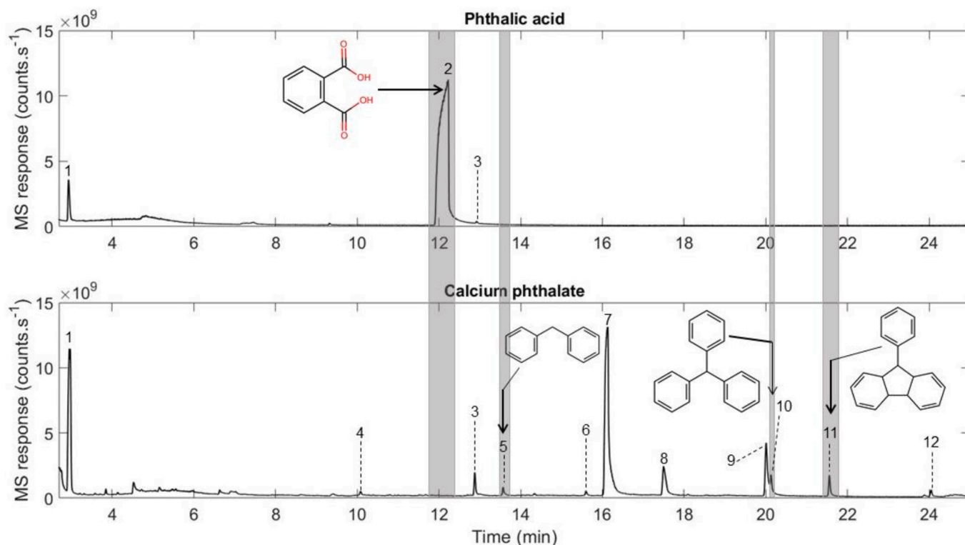
Fig. 4. Chromatograms obtained from the pyrolysis ( 35\text{ }^{\circ}\text{C}\cdot\text{min}^{-1} ramp, up to 800\text{ }^{\circ}\text{C} ) of phthalic acid (top) and calcium phthalate (bottom) at 1 wt% in fused silica in SAM-like pyrolytic conditions. The grey shading corresponds to molecules unique to the pyrolysis of the acid or unique to that of the salt. (1) benzene, (2) phthalic acid, (3) biphenyl, (4) naphthalene, (5) diphenylmethane, (6) fluorene, (7) benzophenone, (8) fluorenone, (9) anthracenedione, (10) triphenylmethane, (11) fluorene, phenyl-, (12) anthracene, phenyl-.
