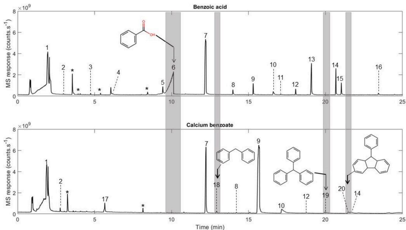
Fig. 3. Chromatograms obtained from the pyrolysis (35 °C·min -1 ramp, up to 800 °C) of benzoic acid (top) and calcium benzoate (bottom) at 1 wt% in fused silica, in SAM-like pyrolytic conditions (35 °C·min -1 ). The grey shading corresponds to molecules unique to the pyrolysis of the acid or unique to that of the salt. (*)artifact of the column (stationary phase bleeding), (1) benzene, (2) toluene, (3) styrene, (4) phenol, (5) naphthalene, (6) benzoic acid, (7) biphenyl, (8) dibenzofuran, (9) benzophenone, (10) fluorenone, (11) Fluorene, methylene-, (12), (14), and (15) terphenyl isomers, (13) anthracenedione, (16) benzantracene, (17) trimethylbenzene, (18) diphenylmethane, (19) triphenylmethane, (20) 9H-Fluorene, phenyl-.
