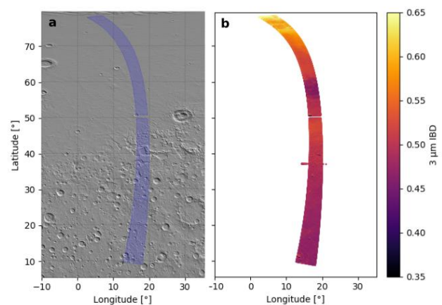
Figure 1 – a. Footprint of 3 OMEGA cubes (#2, 3 and 4) from Mars Express orbit 3747 ( L_s = 147^\circ ), shown on a MOLA relief shaded map. b. 3 \mu\text{m} IBD variations associated with these observations.
