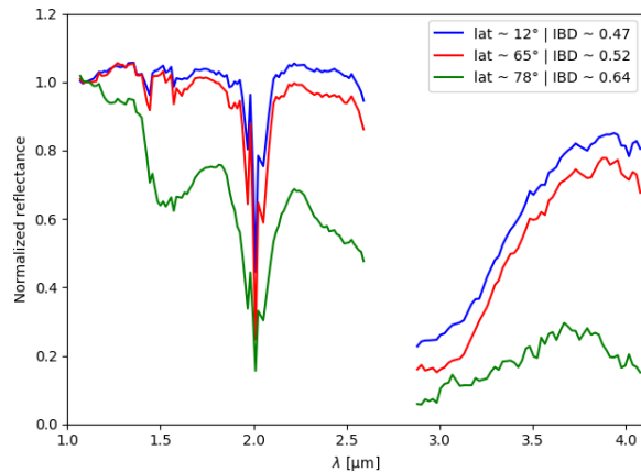
Figure 2 – OMEGA reflectance spectra, corrected for thermal contribution, extracted from observations of Figure 1 at 3 different latitudes. Each spectrum is an average of 2000 OMEGA/MEx spectra. The spectrum at 78°N (green) contains a strong 1.5 μm feature indicative of surface water ice from the perennial cap. The two other spectra are taken outside the main polar cap. Spectra are not corrected for atmospheric (gas and aerosols) contribution.
