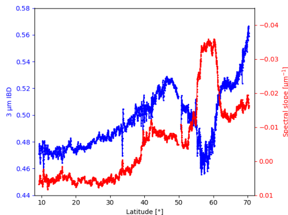
Figure 3 – Latitudinal variations of the IBD (blue) and the 1 – 2.5 μm spectral slope (red), from the OMEGA observations of the orbit 3747.
