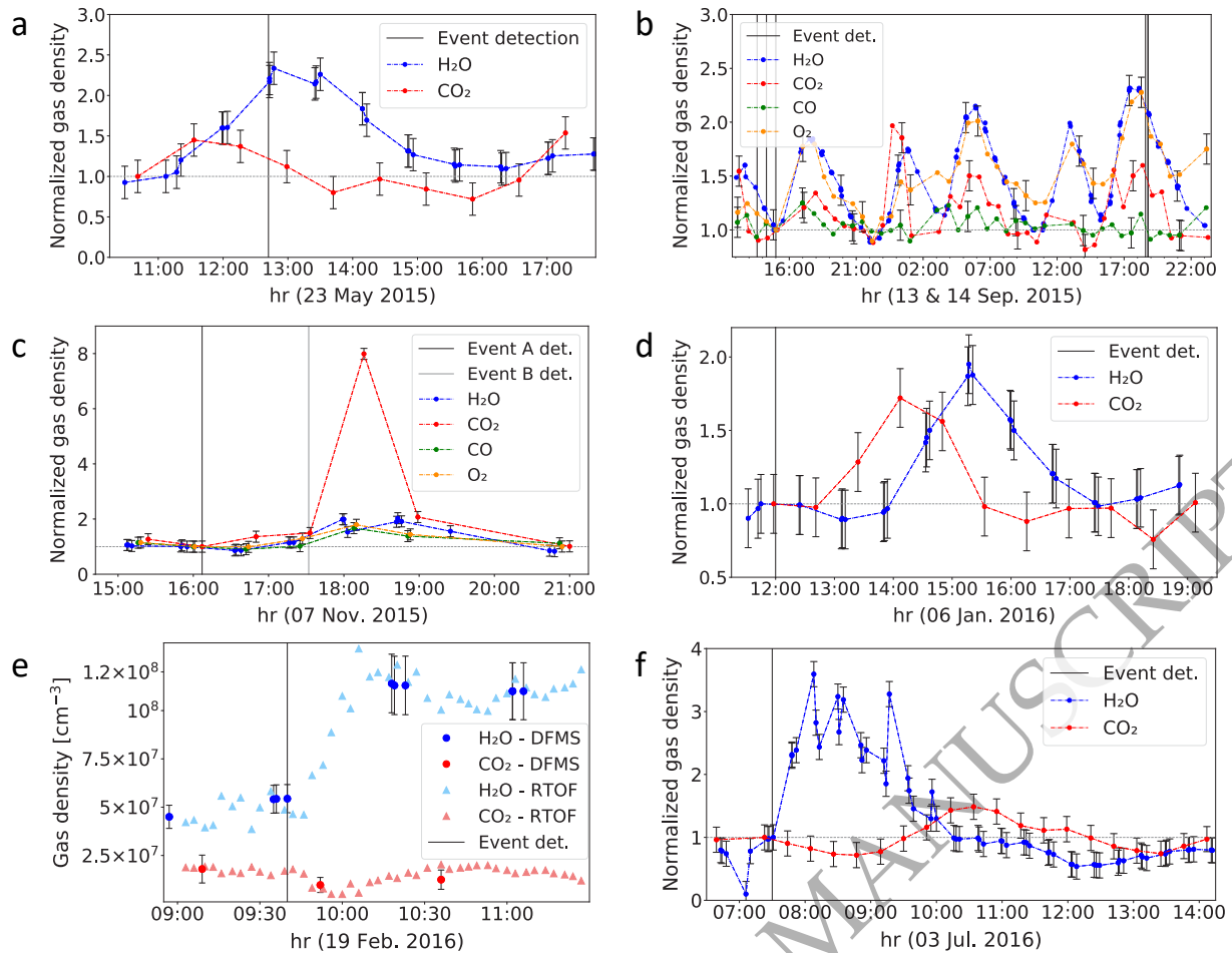
Figure 6. Gas densities of \text{H}_2\text{O} and \text{CO}_2 normalised to their quiescent coma levels during the outbursts of (a) 2015 May 23, (b) 2015 September 13 and 14, (c) 2015 November 7, (d) 2016 January 6, and (f) 2016 July 3 measured with ROSINA/DFMS. Panel (e) represents the absolute gas densities of \text{H}_2\text{O} and \text{CO}_2 for the outburst observed on 2016 February 19 measured with both the ROSINA/DFMS and the ROSINA/RTOF. The absolute densities are displayed in panel (e) to underline that both instruments acquired the same absolute results and no normalisation or instrument effect occurred. Error bars show uncertainties of the DFMS measurements. In panel (b), uncertainties are only displayed on every 15 th data point for \text{H}_2\text{O} and on every 5 th data point for the other volatiles to improve readability. RTOF uncertainties are not shown because they are of the order of the symbols. The vertical lines represent the times when the dust events have initially been detected by the Rosetta cameras (the dust events could have started up to 5 to 30 minutes before). The grey horizontal lines show the quiescent level of the normalised data.
