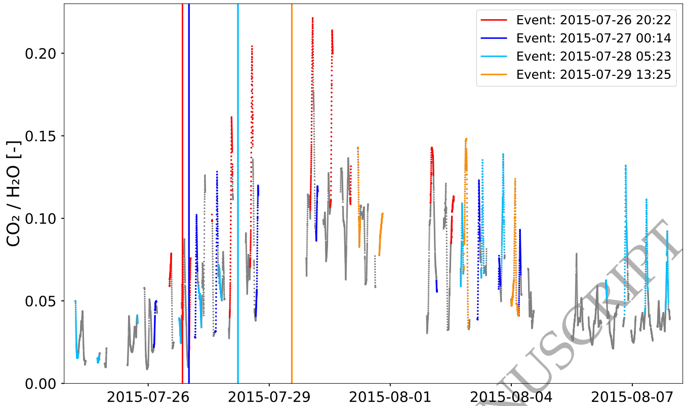
Figure 1. Ion count ratio from ROSINA/DFMS for \text{CO}_2 relative to \text{H}_2\text{O} from 2015 July 24 until August 8. The coloured data points show measurements taken when the Rosetta spacecraft was flying over the identified source location of the respective event observed by the Rosetta cameras at the time marked by the corresponding vertical line. For a better representation, only a part of the summer fireworks’ period (Vincent et al. 2016a) and only four distinct events are shown. The first three events were morning outburst whereas the last event (orange) was a midday outburst.
