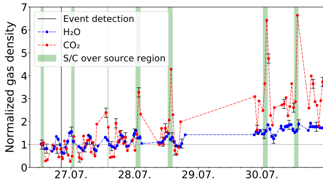
Figure 2. Gas densities of H 2 O and CO 2 normalised to their quiescent coma levels during the CO 2 enhanced outburst from 2015 July 26 measured with ROSINA/DFMS. The quiescent values have been retrieved a few hours before the dust event. Uncertainties are only shown on every 10 th data point for H 2 O and on every 5 th data point for the other volatiles to improve visibility. The vertical line represents the time when the event has been detected by the Rosetta cameras and the green areas represent the time when the spacecraft was above the considered outburst source region. The grey horizontal line shows the quiescent level of the normalised data. The continuous increase of both H 2 O and CO 2 is due to the spacecraft’s movement across the generally more active Southern hemisphere of 67P during that time.
