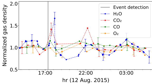
Figure 5. Gas densities of H 2 O, CO 2 , CO, and O 2 normalised to their quiescent coma levels during the water enhanced outburst 2015 August 12 measured with ROSINA/DFMS. The quiescent values have been retrieved a few hours before the dust event. Uncertainties are only shown on every 10 th data point for H 2 O and on every 5 th data point for the other volatiles to improve visibility. The vertical line represents the time when the event has been detected by the Rosetta cameras. The grey horizontal line shows the quiescent level of the normalised data.
