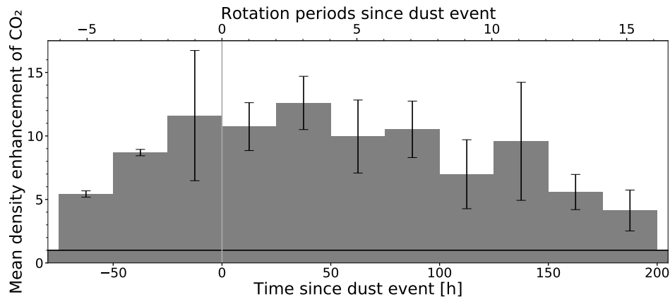
Figure 3. Weighted mean density enhancement for \text{CO}_2 during the summer fireworks outburst events as a function of time. The enhancement is the maximum of the ratio \text{CO}_2/\text{H}_2\text{O} during each fly-over divided by the same ratio in the quiescent coma. Time zero represents the time when the dust event has been observed with the Rosetta cameras (timing precision is 5 to 10 minutes). The horizontal line shows the unchanged ratio (enhancement factor of 1). Only events exhibiting a \text{CO}_2 enhancement are considered.
