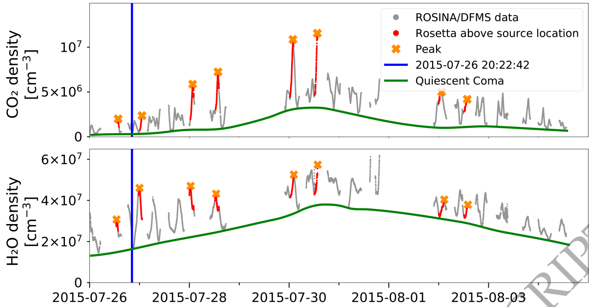
Figure A3. Typical ROSINA/DFMS densities of CO 2 and H 2 O from 2015 July 26 until 2015 August 4 to show the analysis approach for the event on 2015 July 26, 20:22 UTC. To calculate the enhancement each time Rosetta was above the source location (i.e., for all phases with red measurement points), the peak value (orange cross) of CO 2 has been selected and corrected to the quiescent coma (green line). The same has been done for H 2 O for the time when CO 2 showed its maximum. The peak values are slightly shifted in time due to the mass scanning nature of the instrument. These time shifts, on the order of a few minutes, do not affect the enhancement calculations as the timescales associated to Rosetta passing above the active region is substantially longer. The enhancement is then calculated based on Equation 1 .
