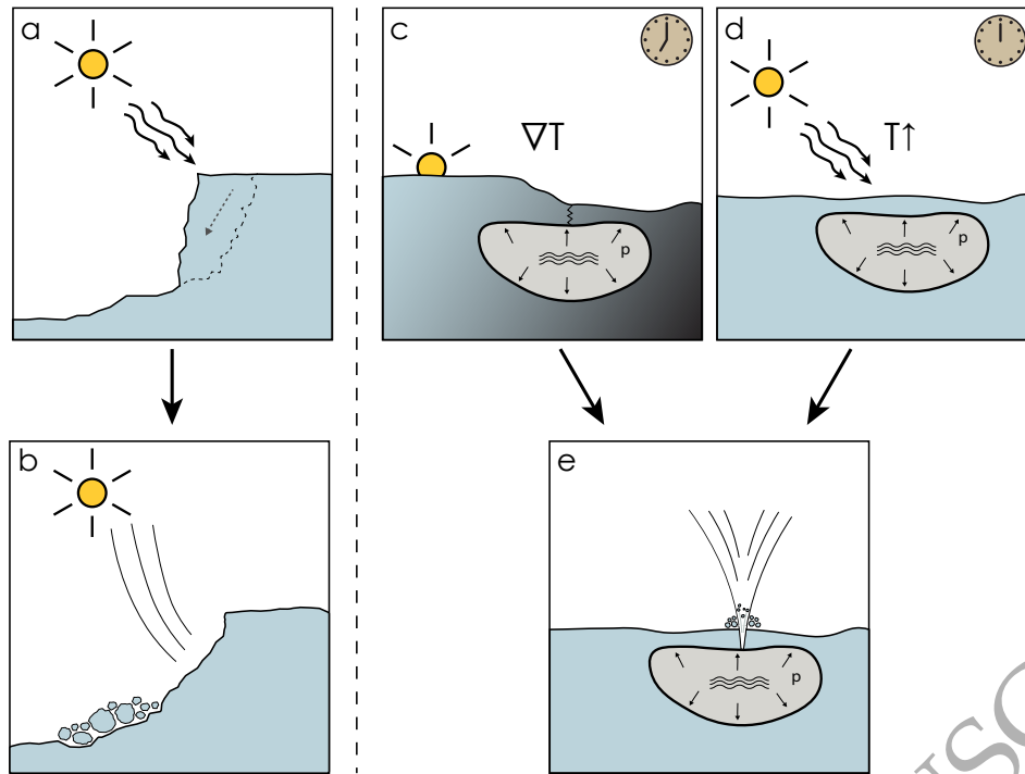
Figure 7. Schematics of outburst trigger mechanisms: 1) Cliff collapse: a) Solar illumination heats up a cliff that collapses due to thermal formation of small cracks. The collapse releases dust from the surface seen as an outburst in the visible range of the cameras. b) After the collapse, freshly exposed water ice sublimates and the released gas can be measured by the Rosetta instruments. 2) Gas pockets: c) A large temperature gradient due to the local sunrise induces cracks where sub-surface pressure pockets containing volatiles can release their pressurised gas leading to an outburst. d) The high temperature at local noon heats up the surface and sub-surface. This increases the pressure in the gas pockets until the pressure is high enough to overcome the tensile strength of the surface inducing an outburst. e) When the surface cracks are large enough or the pressure has been increased enough as shown in c) and d), the pressurised gas pockets violently release dust and gas. Panels c) – e) only show the triggering mechanism of the event and do not display the continuous outgassing before and after the \text{CO}_2 -driven outbursts.
