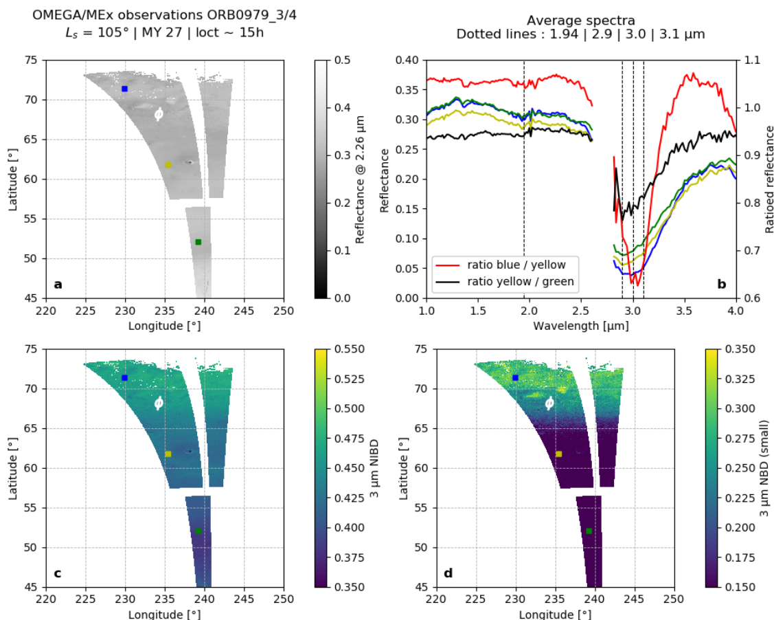
Figure 1 – Maps of OMEGA cubes #3 & #4 from orbit 979 showing the surface reflectance at 2.26 \mu\text{m} (a), the 3 \mu\text{m} NIBD (c) and the coverage of the additional 3 \mu\text{m} component (d). The white “Φ” indicates the position of the Phoenix lander. The blue, yellow and green spectra of the panel (b) are averaged on a square of 3 \times 3 pixels whose position are indicated by the colored squares on panels (a), (c) & (d). We observe on panel (b) that the evolution between 60^\circ\text{N} and 70^\circ\text{N} (purple line) is very different than between 50^\circ\text{N} and 60^\circ\text{N} (black line) with a narrow signature centered around 3 \mu\text{m} , which results in a shift of the position of the maximum of absorption of the widespread Martian 3 \mu\text{m} band from 2.9 \mu\text{m} (yellow & green) to 3.0 \mu\text{m} (blue).
