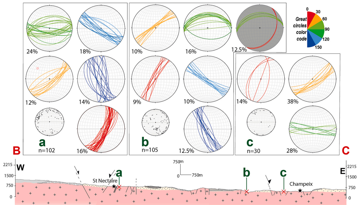
Fig. 8. Stereographic diagrams (equal area projection, lower hemisphere) of fractures populations measured in 3 sites analyzed along the cross-section Saint Nectaire-Champeix, East of the Mont-Dore horst. Small stereographic diagrams of the full population. The grey stereographical projection in the site b corresponds to conjugate shear fractures (see text for explanation and Fig. 10b). Locations in Fig. 7.
