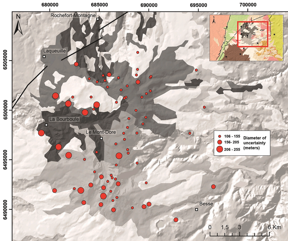
Fig. 12. Location and diameters of uncertainty of 74 volcanic vents identified over the MDVF based on Brousse and Tempier (1981), Brousse et al. (1990), Lavina (1985) and our field work. Because of their limited number, vents related to the Caldera unit are not considered.
