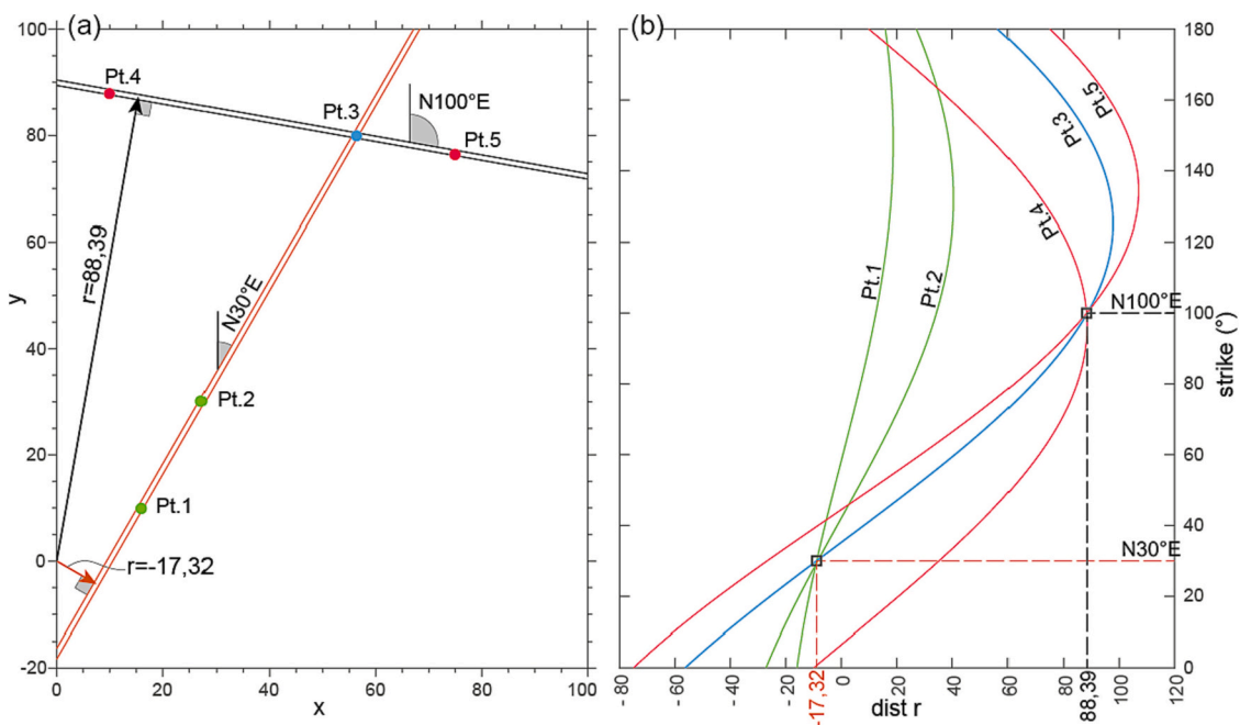
Fig. 4. The Hough transform method used to detect points alignment by image analysis. a – Example of two sets of points that are aligned at N100°E (red and blue dots) and N30°E (green and blue dots) respectively. b – The resulting Hough transform projection plane obtained from the map configuration in a; location and direction of the two alignments are detected where the sinusoidal curves (each corresponding to one point in the map) intersect. (For interpretation of the references to colour in this figure legend, the reader is referred to the web version of this article.)
