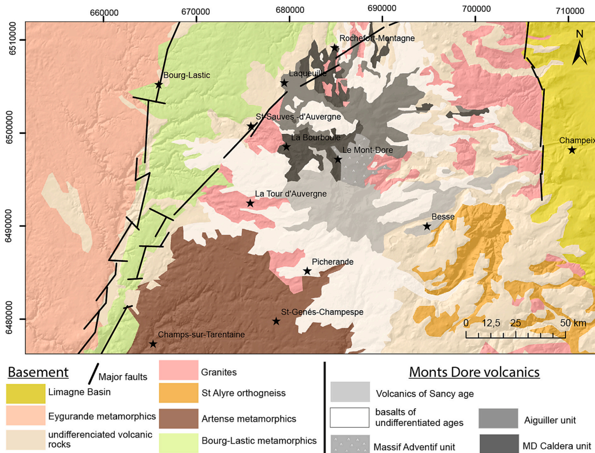
Fig. 3. Simplified geological map issued from Fig. 1 and in which each unit of both the basement and the Mont Dore Volcanic Field have been individualized. See text for the description.
