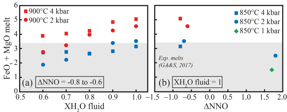
Figure 4. Influence of (a) the mole fraction of \text{H}_2\text{O} in the experimental fluid ( \text{XH}_2\text{O} fluid) and of (b) \Delta\text{NNO} (deviation from the Ni–NiO oxygen buffer at the same T and P ) on concentrations of \text{FeO}_t + \text{MgO} in experimental silicic melts. Data from Cadoux et al. (2014). In panel (a), the \Delta\text{NNO} range indicated pertains to charges with \text{XH}_2\text{O} fluid = 1. Charges with \text{XH}_2\text{O} fluid < 1 have slightly lower \Delta\text{NNO} . In panel (b), only charges with \text{XH}_2\text{O} fluid = 1 are shown. Melts are rhyodacitic to rhyolitic and at equilibrium with orthopyroxene + ilmenite as Fe- and Mg-saturating phases for \Delta\text{NNO} < 0 and orthopyroxene + magnetite for \Delta\text{NNO} > 0 . At 1 kbar, amphibole joins orthopyroxene + magnetite. The grey domain is the field of experimental partial melts from García-Arias and Stevens (2017). Melts from Cadoux et al. (2014) have \text{FeO}_t + \text{MgO} concentrations (maximum 5.06 wt %) that exceed the maximum (3.41 wt %) of reference experimental melts (grey domain), especially at 900 °C for \text{XH}_2\text{O} fluid > 0.7 and at 850 °C for \Delta\text{NNO} < 0.5 . Note that melt \text{FeO}_t + \text{MgO} concentrations continue to increase below \Delta\text{NNO} < -1 . There is no apparent necessity to limit the \text{FeO}_t + \text{MgO} of crustal silicic melts to \sim 3.5 wt % maximum (García-Arias and Stevens, 1997). Additional examples in the literature of experimental melts with \text{FeO}_t + \text{MgO} > 3.5 wt % include Gardien et al. (1995).
