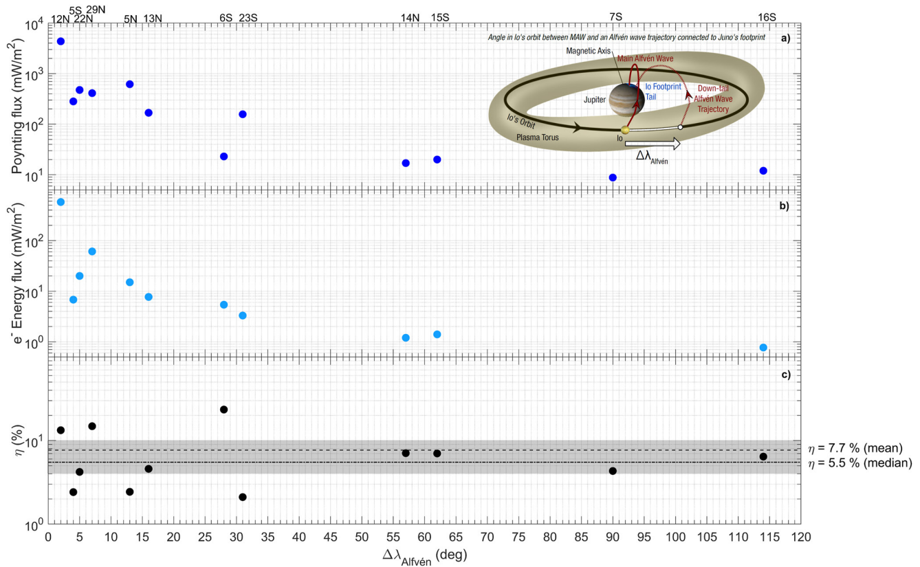
Figure 2. (a) Poynting fluxes (PFs), measured locally, as a function of \Delta\lambda_{\text{Alfvén}} . (b) Peak electron energy fluxes, measured locally, as a function of \Delta\lambda_{\text{Alfvén}} . (c) Efficiency, or fraction of electron energy to PFs, as a function of \Delta\lambda_{\text{Alfvén}} . The gray rectangle is the range of efficiencies (4%–10%) theoretically computed by Hess et al. (2010) for filamented waves obtained through a turbulent cascade. (inset) Illustration of how \Delta\lambda_{\text{Alfvén}} is defined (Szalay, Allegrini, et al., 2020b).
