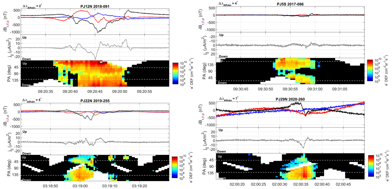
Figure 1. (top panels) Time series of magnetic field perturbations, \delta B , when Juno crossed flux tubes connected to Io's orbit. All are presented on the same scale. The perturbations were computed by subtracting the JRM33 internal magnetic field model from the measured magnetic field. We further subtract the residuals from the interval average to bring the baseline field close to the zero line. The coordinate system is the radial-theta-phi with respect to Jupiter's JRM33 dipole axis. Perturbations of \delta B_\phi are indicative of field-aligned currents with the sign of the gradients related to the current direction, that is, toward or away from Jupiter. (middle panels) Computed 1s-averaged field-aligned current densities from \delta B using Equation 1. (bottom panels) Pitch angle spectrograms of background (non-Io) subtracted differential energy flux. Overlaid as white dashed lines are the loss cone angles.
