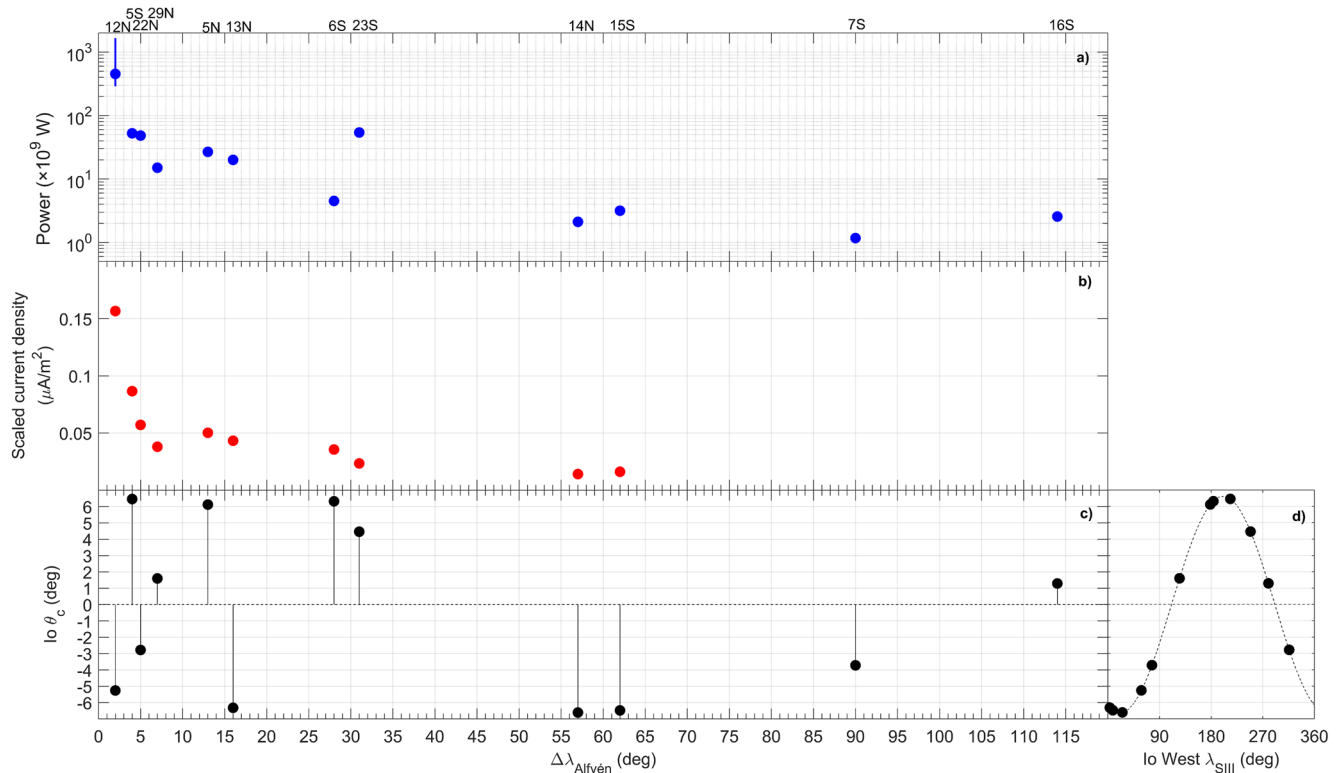
Figure 3. (a) Power as a function of \Delta\lambda_{\text{Alfvén}} . The power is calculated by multiplying the local Poynting flux (in \text{mW}/\text{m}^2 ) by the area of Io using an effective radius of 1.3R_{\text{Io}} , and scaling to Io's orbit along the magnetic flux tube as B_{\text{Io}}/B_{\text{Juno}} . The blue vertical line on the PJ12N-MAW event represents the range of powers theoretically modeled by Saur et al. (2013). (b) Peak (of the modulus) of 1 s-averaged field-aligned current densities ( j_{\parallel} ), scaled to Io's orbit, as a function of \Delta\lambda_{\text{Alfvén}} . (c) Estimate of Io's centrifugal latitude at the time when the initial Alfvén wave was launched. (d) Estimate of Io's System-III west longitude corresponding to its centrifugal altitude in (c).
