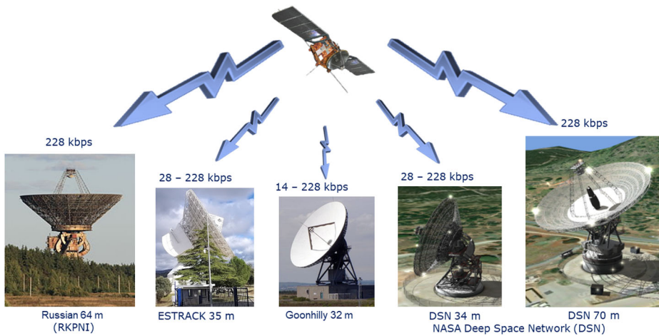
Fig. 15 Ground Station Networks and Capabilities. For the smaller antennas, the variable bitrate (in kilobits per second) depends on the Earth-Mars distance
