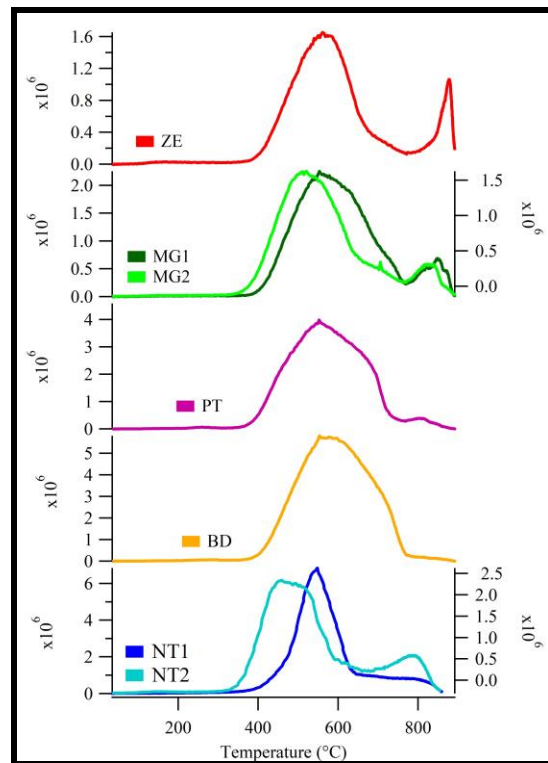
Fig. 2. \text{SO}_2 ( m/z 64) releases from samples drilled throughout the upper GT and clay-sulfate transition region. Units in counts per second.
