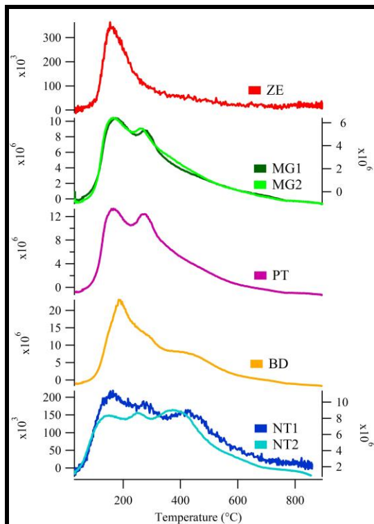
Fig. 1. \text{H}_2\text{O} ( m/z 17; m/z 19 for NT1) releases from samples drilled throughout the upper GT and clay-sulfate transition region. Units in counts per second.
