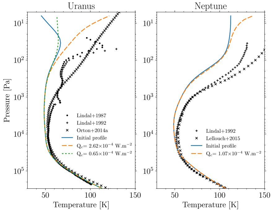
Figure 12: Scenario with no hazes including heat conduction. Left: simulated temperature profiles on Uranus for the UC1 (dashed orange curve) and UC2 (dotted green curve) thermospheric conduction scenarios. Right: simulated temperature profiles on Neptune for NC1 (dashed orange curve) thermospheric conduction scenario. The solid blue line is the initial case without conduction (section 3). The black symbols are the observed temperatures described in fig.2.
