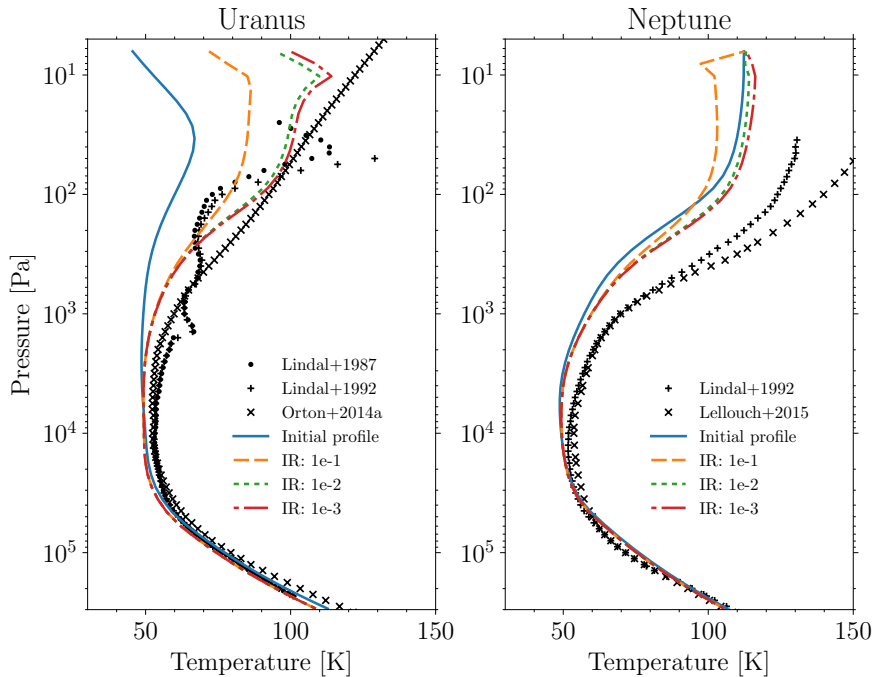
Figure 5: Simulated temperature profiles of Uranus (left) and Neptune (right) with the Irwin et al. (2022) haze scenario for three different values of the absorption coefficient in the thermal infrared. The orange dashed line is the case with an imaginary index of 10^{-1} in the thermal infrared, the green dotted line is the 10^{-2} case and the red dotted-dashed line is the 10^{-3} case. For n_i lower than 10^{-3} in the thermal infrared, we obtain the same temperature profile as the case at 10^{-3} . In comparison, the temperature reached without aerosols is added as a blue line and the different observations are shown in black as described in fig.2.
