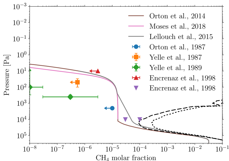
Figure 7: Methane volume mixing ratio in the atmosphere of Uranus estimated by different observations and models. The dotted line represents the liquid saturated \text{CH}_4 vmr calculated from Lindal et al. (1987) temperature profile and the dashed line is the ice saturated \text{CH}_4 vmr. The nominal \text{CH}_4 vmr profile used in our model is Lellouch et al. (2015) below the 100 Pa level and Moses et al. (2018) above the 100 Pa level.
