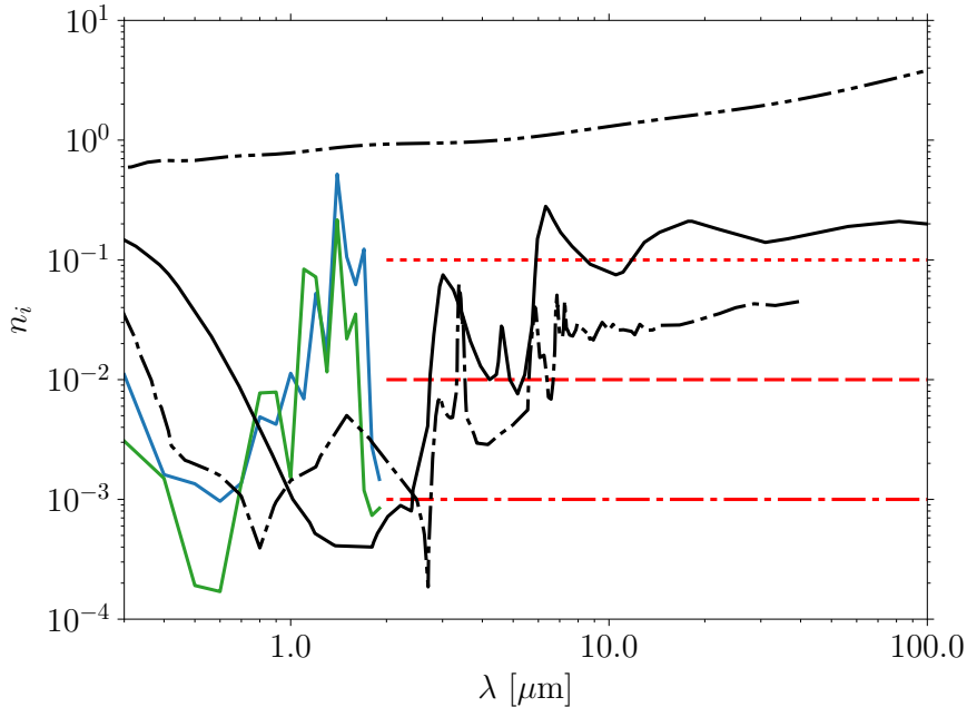
Figure 3: Uranus: Imaginary refractive indices for Uranus. The blue line corresponds to the vertically extended photochemical haze and the green line to the concentrated haze located near the \text{CH}_4 condensation level from Irwin et al. (2022). Three different ad hoc values ( 1 \times 10^{-1} , 1 \times 10^{-2} , 1 \times 10^{-3} ) in the thermal infrared ( > 2 \mu\text{m} ) are added (red lines). For reference, refractive indices of tholins (Khare et al., 1984), ice tholins (Khare et al., 1993) and black carbon (Jäger et al., 1998) are also shown in solid, dotted-dashed and double dotted-dashed black lines respectively.
