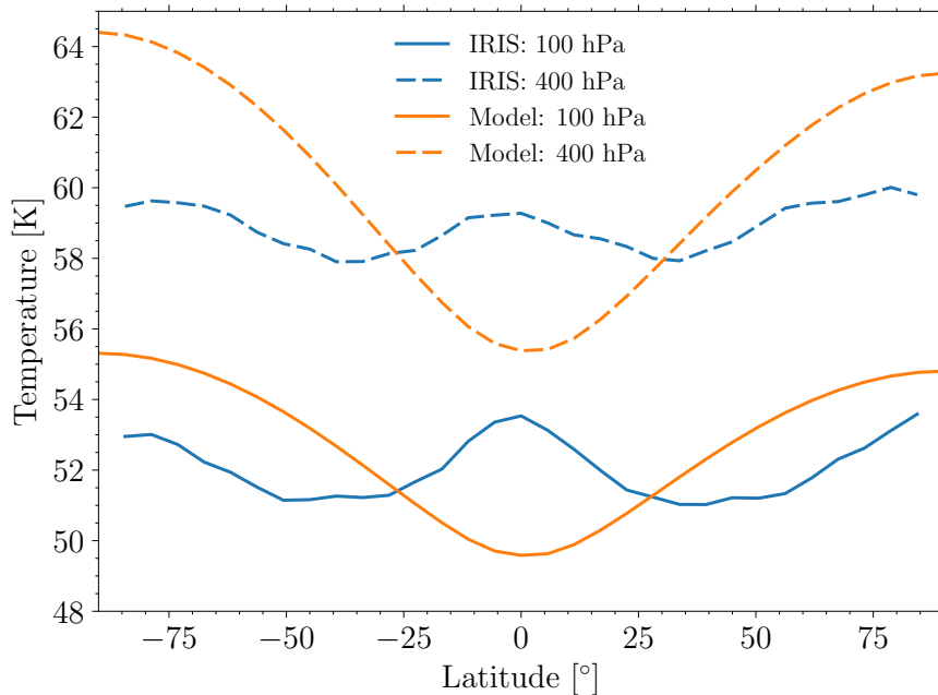
Figure 19: Uranus: Comparison of the temperature retrieved (blue line) from Voyager 2/IRIS experiment (Orton et al., 2015) and the simulated temperature (orange line) at 100 hPa (solid line) and 400 hPa (dashed line). Uncertainties from the spectral inversion of IRIS data are lower than 1 K.
