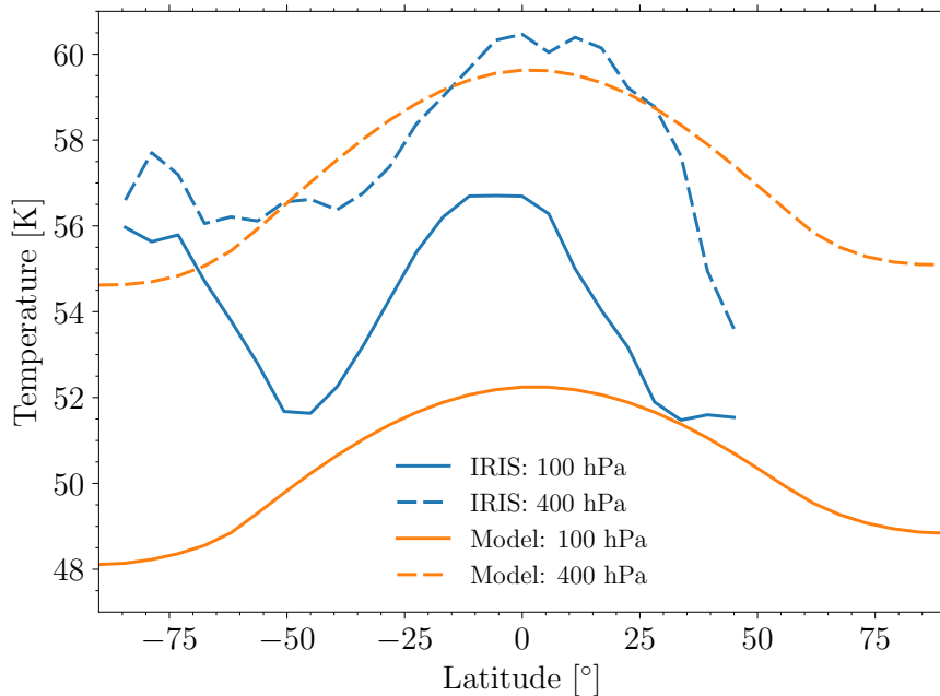
Figure 21: Neptune: Comparison of the temperature retrieved (blue line) from IRIS experiment (Fletcher et al., 2014) and the temperature simulated (orange line) at 100 hPa (solid line) and 400 hPa (dashed line). Uncertainties from the spectral inversion of IRIS data are lower than 1 K.
