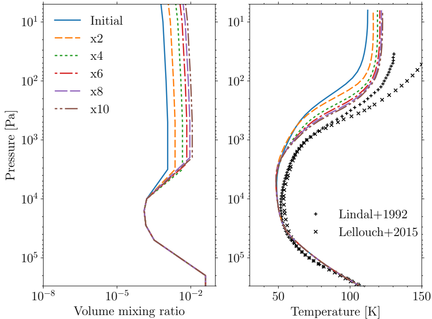
Figure 10: Left: \text{CH}_4 vmr profile on Neptune with the nominal \text{CH}_4 vmr profile (solid blue line, see section 3), or with that abundance multiplied 2 (short dashed orange curve), 4 (dotted green curve), 6 (dotted-dashed red curve), 8 (long dashed violet curve) and 10 (double dotted-dashed maroon curve) above the methane condensation level. Right: the corresponding simulated temperature profiles. The black symbols correspond to the observed temperatures described in fig.2 .
