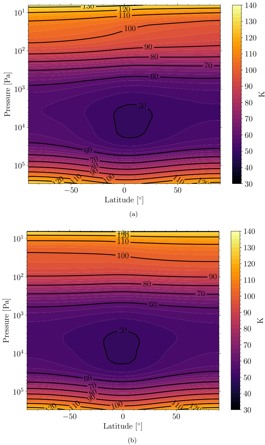
Figure 14: Uranus: Vertical cross sections of temperature at spring equinox ( L_s=0^\circ ) (a) and northern summer solstice ( L_s=90^\circ ) (b). The temperature observed at autumn equinox and winter solstice is almost similar (because of its slightly non circular orbit) as spring equinox and summer solstice but the maximum/minimum temperature is reversed in latitude (fig.16).
