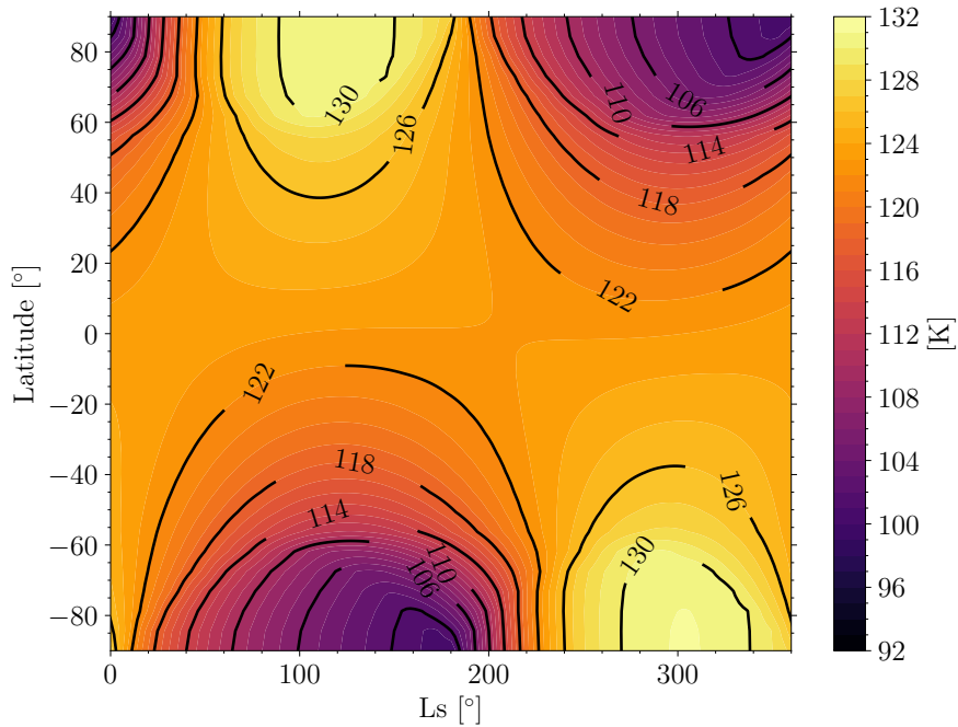
Figure 17: Evolution of the simulated temperature at 10 Pa on Neptune during one Neptunian year.
