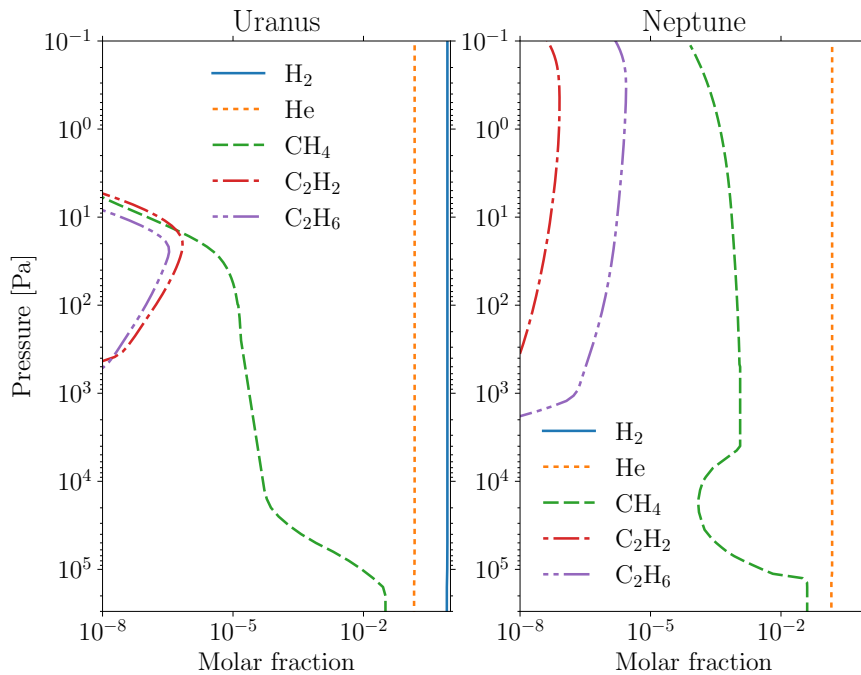
Figure 1: Vertical molar fraction of the gases on Uranus (left) and Neptune (right) used by the model. Collision-induced absorptions/emissions of \text{H}_2 and He contribute to radiative heating/cooling throughout the entire atmospheric column, as absorption/emission by methane (except on Uranus, where its abundance becomes insignificant at pressures below \sim 10 Pa). The other hydrocarbons are active only in the stratosphere for pressures between \sim 1 hPa and \sim 7 Pa on Uranus and below than \sim 10 hPa on Neptune.
