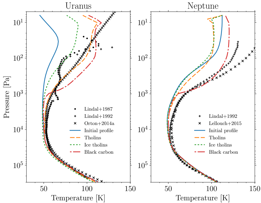
Figure 6: Simulated temperature profiles of Uranus (left) and Neptune (right) with the Irwin et al. (2022) haze scenario but with different optical indices. The orange dashed line is the case where the Irwin et al. (2022) optical indices are replaced by those of tholins (Khare et al., 1984) and the green dotted line corresponds to ice tholins (Khare et al., 1993). The red dotted-dashed line is the temperature simulated with an adhoc black carbon dust layer located between 5 and 1000 Pa. In comparison, the temperature reached without aerosols is displayed as a blue line and the different observations are shown in black as described in fig.2.
