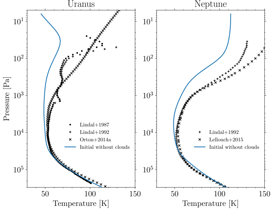
Figure 2: Temperature simulated by the nominal model in blue on Uranus (left) and Neptune (right) at the same latitude and solar longitude as the observations (see text). Observed temperature profiles are from Lindal et al. (1987) (black dots), Lindal (1992) (black plus), Orton et al. (2014) (black cross) for Uranus and Lellouch et al. (2015) (black cross) for Neptune.
