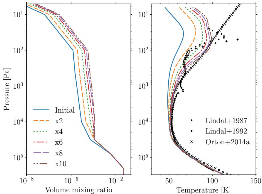
Figure 9: Left: CH 4 vmr profile on Uranus (solid blue line, see section 3), with 2 (short dashed orange curve), 4 (dotted green curve), 6 (dotted-dashed red curve), 8 (long dashed violet curve) and 10 (double dotted-dashed maroon curve) times the nominal abundance. Right: the corresponding simulated temperature profiles. The black symbols are the observed temperatures described in fig.2 .
