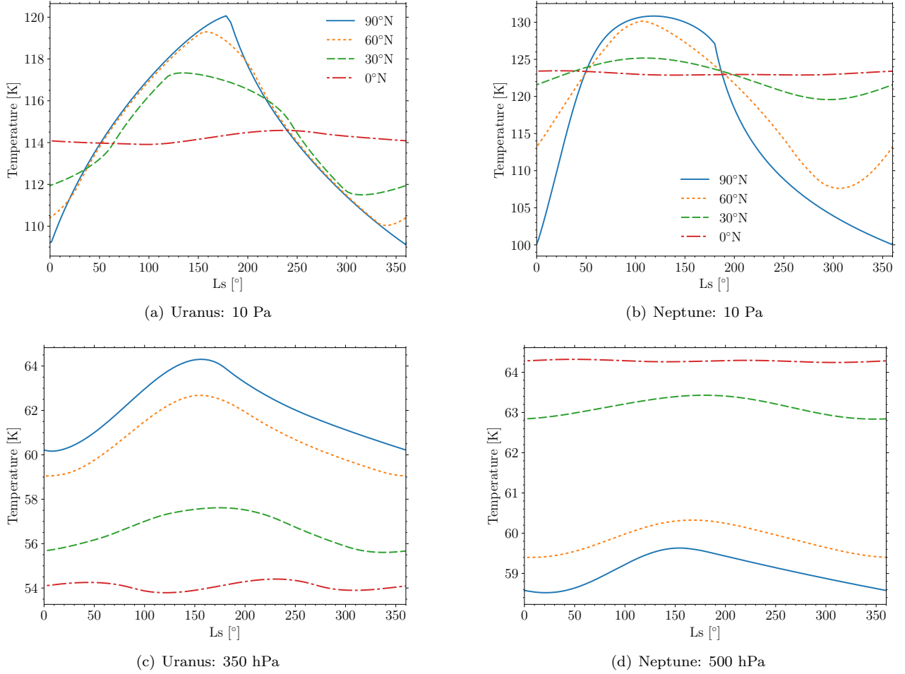
Figure 18: Evolution of temperature during one planetary year on Uranus (left) at 10 Pa (a) and 350 hPa (c) and on Neptune (right) at 10 Pa (b) and 500 hPa (d) for a latitude of 90°N (blue solid line), 60°N (orange dotted line), 30°N (green dashed line) and 0° (red dashed-dotted line).
