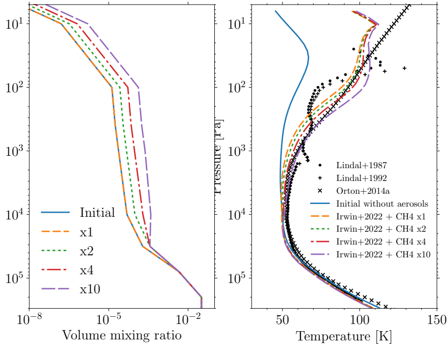
Figure 11: Left: CH 4 vmr profile on Uranus (blue line and short dashed orange line) or with that abundance multiplied by a factor of 2 (dotted green line), 4 (dotted-dashed red line), 10 (long dashed violet line). Right: the corresponding simulated temperature profiles with the Irwin et al. (2022) haze scenario. The solid blue line corresponds to the initial case without hazes (see section 3) with a nominal CH 4 vmr profile. The black symbols are the observed temperatures described in fig.2.
