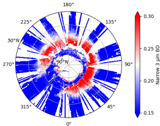
Figure 2 – Composite OMEGA map of the distribution of the narrow 3\ \mu\text{m} band depth in the Martian north polar regions during the northern summer of MY 27 ( L_s = 98^\circ - 132^\circ ). Adapted from [7].
