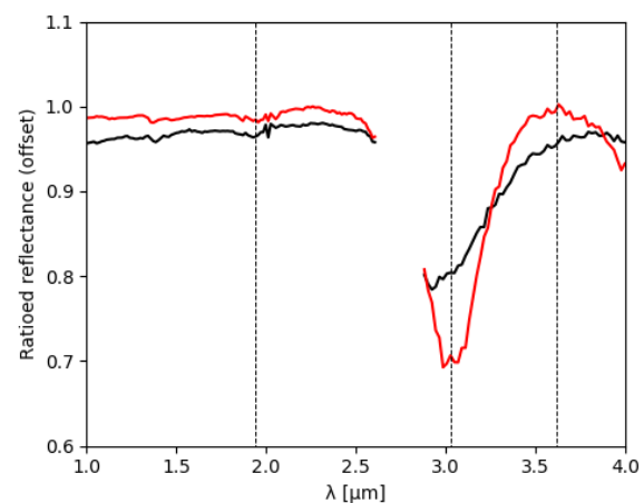
Figure 1 – Typical averaged spectral ratio associated with the 3 \mu\text{m} northern ring ( \sim 70^\circ\text{N} / 63^\circ\text{N} , red) compared to a spectrum of the standard evolution outside the ring ( 60^\circ\text{N} / 50^\circ\text{N} , black). Adapted from [7].
