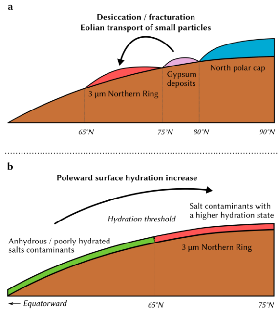
Figure 3 – Schematic drawings of two possible scenarios for the formation of the 3\ \mu\text{m} northern ring. Adapted from [7].
