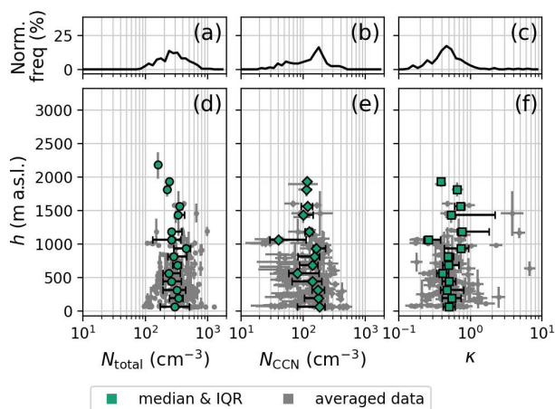
Figure 14. Relative occurrence of the (a) total aerosol particle number concentration N_{\text{total}} , (b) cloud condensation nuclei (CCN) number concentration N_{\text{CCN}} , and (c) CCN hygroscopicity \kappa . Vertical binned averages of (d) N_{\text{total}} , (e) N_{\text{CCN}} , and (f) \kappa . P6 research flights RF08 to RF13 are considered.
