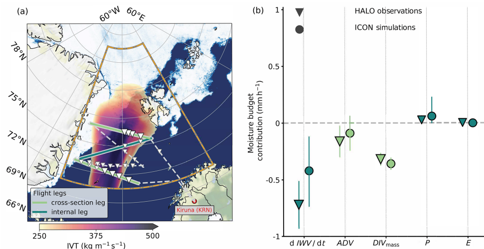
Figure 9. Warm-air intrusion (WAI) on 15 March 2022. (a) HALO flight pattern (dashed gray lines and thick colored lines) and ICON (Icosahedral Nonhydrostatic) model domain (framed by the dashed orange line) for the WAI sampled during RF05. Along the two cross-flow flight sections (thick light green lines), dropsonde observations are indicated by large triangles, whereas small triangles represent the dropsonde releases during the remaining flight sections. The internal leg is indicated by the solid blue line. For the ICON domain, simulated integrated water vapor transport (IVT) values are illustrated in red. (b) For the eastern part of the flight pattern, the moisture budget components from the HALO observations (triangles) are compared to those simulated by ICON (circles) with respect to their contribution to the moisture budget (in \text{mm h}^{-1} ). Moisture advection (ADV), mass divergence ( \text{DIV}_{\text{mass}} ), precipitation rate ( P ), evaporation ( E ), integrated water vapor (IWV), and its temporal tendency ( \text{dIWV}/\text{dt} ) are compared. Vertical lines indicate the uncertainties for each component.
