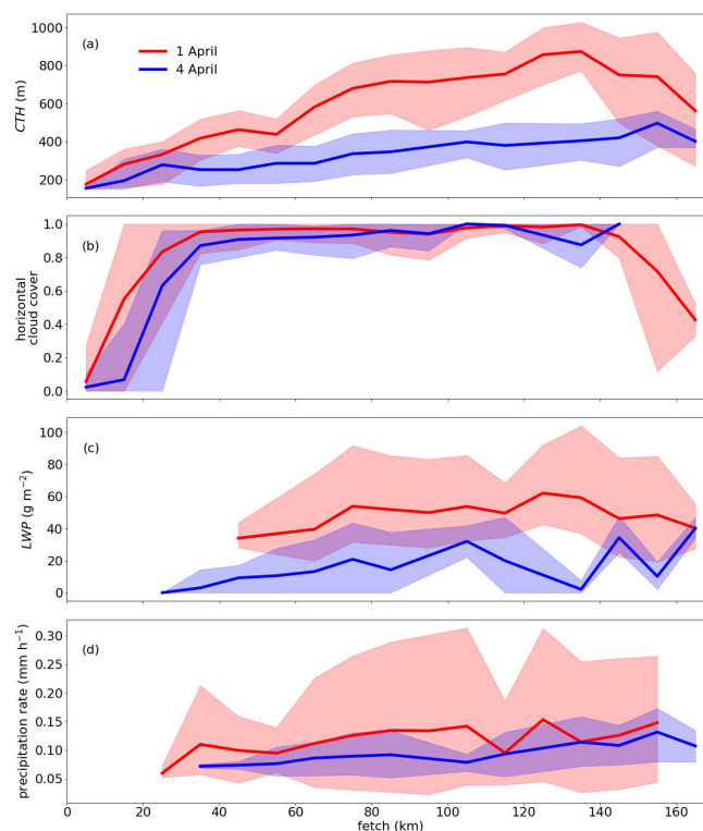
Figure 6. Two cold-air outbreaks (CAOs) – strong on 1 April 2022 and weak on 4 April 2022. Development of macrophysical and microphysical cloud properties as a function of fetch on 1 April (red line; strong CAO) and 4 April 2022 (blue line; weak CAO) as measured with instruments installed on P5. (a) Cloud-top height (CTH), (b) horizontal cloud cover per minute measured by the Microwave Radar/radiometer for Arctic Clouds (MiRAC) and Airborne Mobile Aerosol Lidar (AMALi), (c) liquid water path (LWP), and (d) precipitation rate ( P ) at 150 m height. The shaded areas indicate the 5 % and 95 % quantiles of the distributions as a function of fetch. Figure adapted from Schirmacher et al. (2024).
