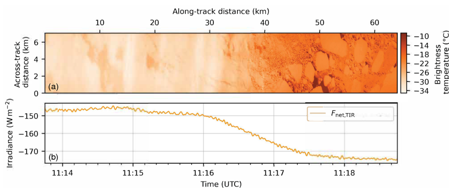
Figure 12. (a) Two-dimensional brightness temperature field measured by VELOX (Video airborne Longwave Observations within six channels) along the flight track in the spectral range of 7.7 to 12 \mu\text{m} . (b) Time series of the thermal infrared (TIR) net irradiance, F_{\text{net,TIR}} = F_{\text{TIR}}^{\downarrow} - F_{\text{TIR}}^{\uparrow} , measured by the Broadband AirCRAFT Radiometer Instrumentation (BACARDI) for the same flight section.
