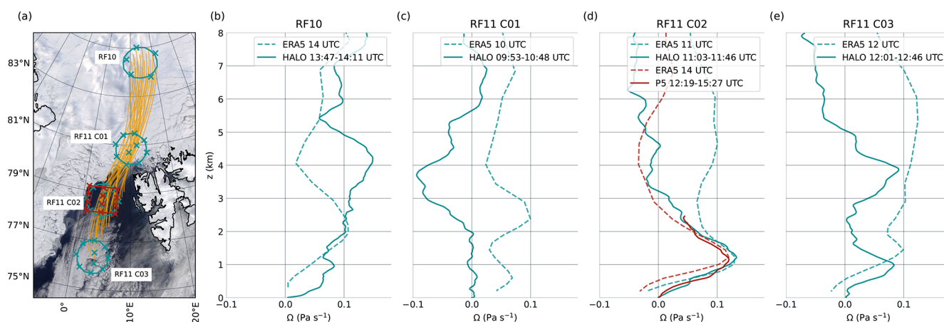
Figure 17. Cold-air outbreak (CAO) on 29 and 30 March 2022. (a) Overview of mesoscale flight patterns flown by HALO (green circles) and P5 (square in a red pattern) sampling a low-level air mass at four locations along its southbound trajectory (yellow lines). Dropsonde launch locations are marked by crosses (green crosses for sondes dropped by HALO; red crosses for sondes dropped by P5). (b–e) Profiles of pressure velocity \Omega calculated from dropsonde data (time of first and last dropsonde launch indicated) released from HALO and P5 (solid lines) and ERA5 reanalysis data (dashed lines).
