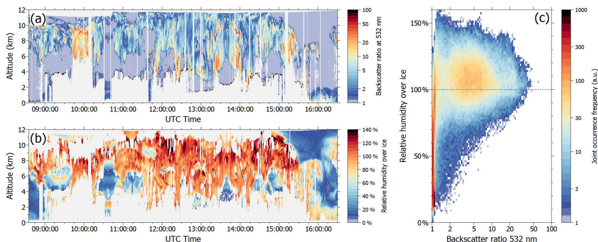
Figure 13. Warm-air intrusion (WAI) on 13 March 2022. Cross section of the (a) backscatter ratio at 532 nm and (b) relative humidity with respect to ice ( RH_i ) for RF03. Panel (c) shows a histogram of the joint occurrence of the RH_i and backscatter ratio at 532 nm. The relative humidity was calculated from WALES water vapor measurements and the model temperature field.
