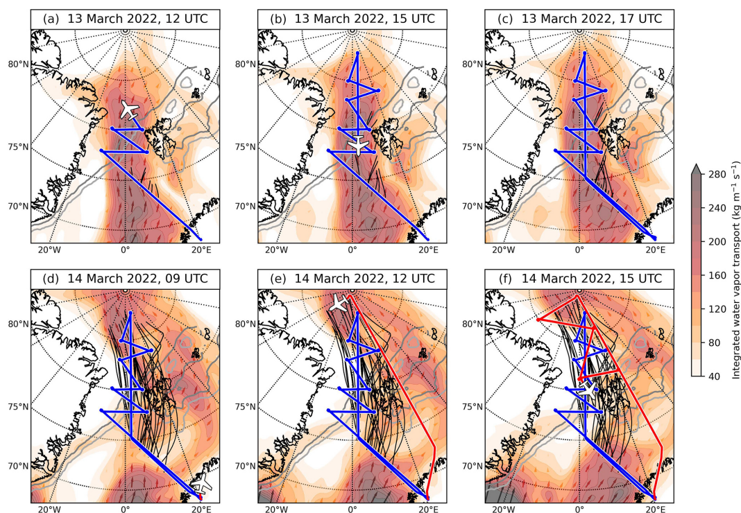
Figure 3. Warm-air intrusion (WAI) on 13 and 14 March 2022. Time series (based on ERA5) of geographic maps, including the integrated water vapor transport (IVT; in red colors, with the length of arrows being proportional to the magnitude of IVT) and the HALO flight tracks on 13 March 2022 (RF03; blue line) and 14 March 2022 (RF04; red line). Black lines indicate the horizontal projections of the evolving matching trajectories.
