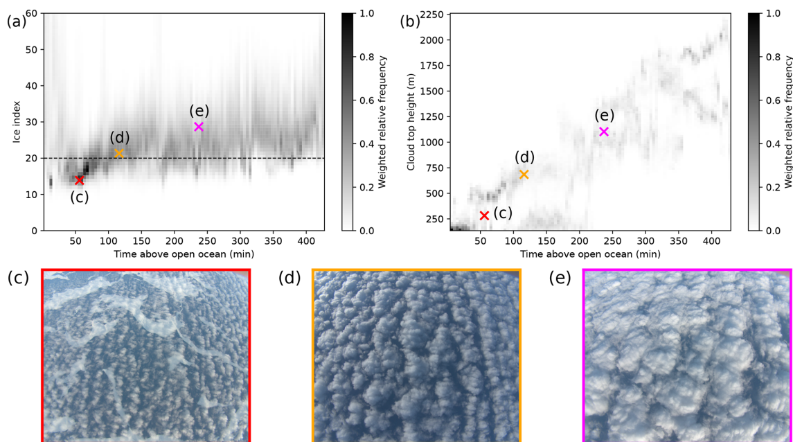
Figure 7. Cold-air outbreak (CAO) on 1 April 2022. (a) Spectral slope phase index (ice index) derived from measurements of the spectrometer of the Munich Aerosol Cloud Scanner (specMACS) as a function of the time the air mass traveled above open ocean. (b) Same as panel (a) but with the cloud-top height (CTH) from a stereographic reconstruction. (c–e) Example RGB (red, green, and blue) images at points indicated by colored crosses in panels (a) and (b) .
