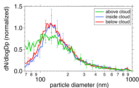
Figure 15. Normalized particle number size distributions of cloud droplet residuals (CDRs; measured inside cloud; blue line) and of ambient aerosol particles (above cloud – green line; below cloud – red line) as measured over open ocean during research flight RF01 with P6 (20 March 2022). The distributions have been normalized with respect to the integrated (total) CDR or ambient particle number concentration.
