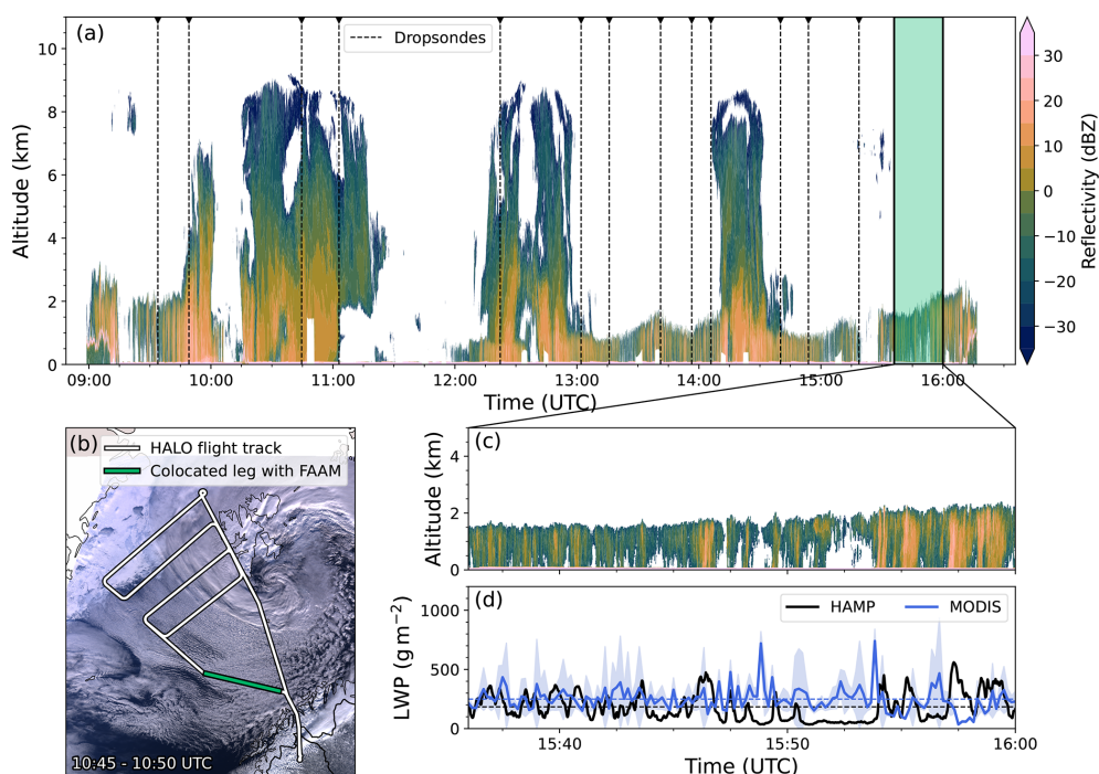
Figure 8. Cold-air outbreak (CAO) on 21 March 2022. (a) Time series of radar reflectivity along the flight track of RF08; the times of dropsonde launches are indicated by vertical dotted black lines. (b) Flight pattern of HALO (white line) and FAAM (green line) during RF08 along the MODIS (Moderate Resolution Imaging Spectroradiometer) overpath (Terra image from 10:45–10:50 UTC; MOD02HKM – Level 1B calibrated radiances). (c) Enlarged view of radar measurements from the last leg which was collocated with FAAM. (d) Time series of the liquid water path (LWP) retrieved from HALO and MODIS (MOD06 – cloud optical properties; two-channel retrieval using band 7 [2.1 \mu\text{m} ] and band 6 [1.6 \mu\text{m} ]) along the enlarged view of the flight track of RF08. Dashed lines show the temporal mean..
