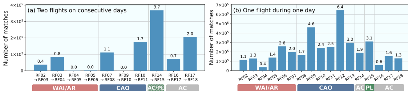
Figure 4. Number of matches for the two scenarios. (a) Two flights on consecutive days and (b) one flight during 1 d. The analysis includes moist- and warm-air intrusions (WAI), atmospheric rivers (AR), marine cold-air outbreaks (CAOs), Arctic cirrus clouds (AC), and polar low (PL) cases.
