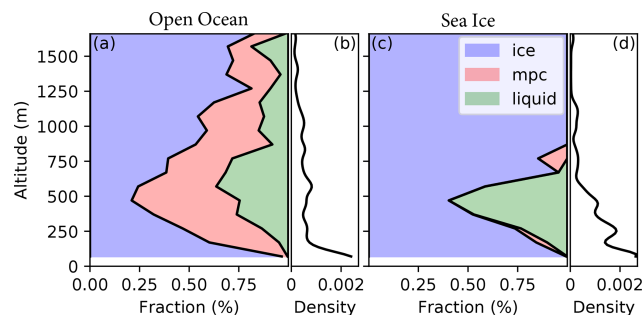
Figure 10. Fraction of detected cloud particle types resolved by altitude. Cloud types (ice is for ice clouds; mpc is for mixed-phase clouds; liquid is for liquid clouds) shown for (a) clouds over the open ocean and (c) clouds over sea ice. Panels (b) and (d) show the distribution of measurements in altitude. Thermodynamic-phase classification was performed according to the algorithm presented by Moser et al. (2023).
