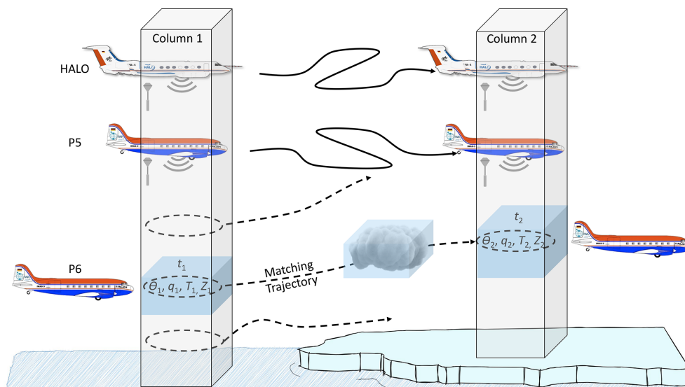
Figure 2. Illustration of the quasi-Lagrangian approach adopted during the HALO–(AC) 3 aircraft campaign. At an initial time t_1 and within atmospheric column 1, an air parcel (blue cube) is observed using remote-sensing and in situ instrumentation installed on HALO, P5, and P6. Trajectories are simulated that describe the movement of the air parcels (dashed arrows). If they cross the flight path of the aircraft at a later time, t_2 , the air parcel can be sampled a second time within atmospheric column 2. This approach enables observing the changes in the properties of the air parcel (for example, \theta , q , T , and Z in the time increment (t_2 - t_1) along its trajectory).
