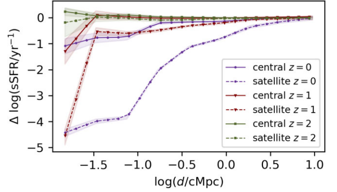
Figure 8. Distance from filaments dependence of the sSFRs’ deviations from the SFMS for centrals (continuous lines) and satellites (dashed lines) for three redshifts: z = 0 (purple), z = 1 (dark red), and z = 2 (green). The lines were obtained by binning the results in terms of distance and interpolating the corresponding medians (i.e. running medians). The shaded regions represent the corresponding standard errors in each bin. The centrals show an increasing suppression of SF activity with time very close to filament centres, with no strong trend at z = 2 while by z = 0 the typical galaxy at the centre of a filament is quenched. The satellites likewise show a strong trend with redshift, with suppression of SF activity extending to quite large distances by z = 0 (see also Fig. 4).
