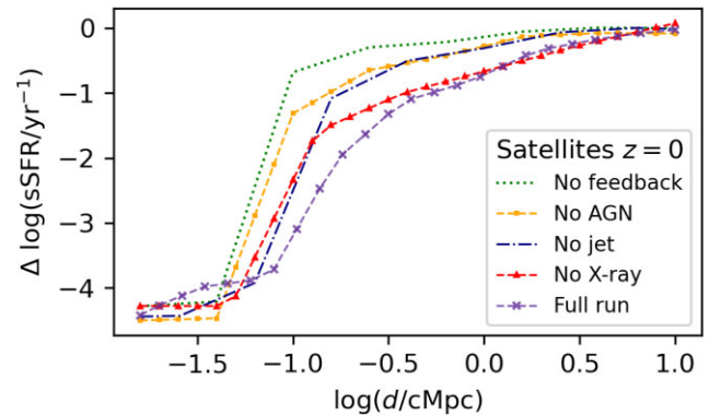
Figure 12. Distance from filaments dependence of the sSFRs' deviations from the SFMS for and satellites at redshift z = 0 , in different feedback scenarios: no feedback (green lines) – same as in Fig. 11; no AGN (yellow lines); no jet (blue lines); no X-ray feedback (red lines); and full run (purple lines) – same as in Figs 8 and 11. The lines were obtained by binning the results in terms of distance and interpolating the corresponding medians (i.e. running medians). Note that no errors are plotted, due to the lines being very close to each other, but the approximate size of the errors in these determinations can be inferred from Fig. 11. Among feedback processes, AGN feedback has the most significant impact on providing extra suppression of sSFR near filaments.
