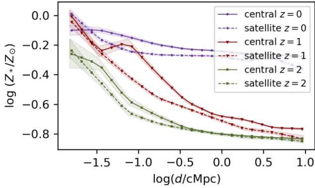
Figure 6. Distance from filaments dependence of stellar metallicities for centrals (continuous lines) and satellites (dashed lines) for three redshifts: z = 0 (purple), z = 1 (dark red), and z = 2 (green). The lines were obtained by binning the results in terms of distance and interpolating the corresponding medians (i.e. running medians). The shaded regions represent the corresponding standard errors in each bin. Galaxies close to filaments are more metal-enriched, the centrals and satellites showing similar behaviours.
