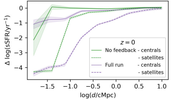
Figure 11. Distance from filaments dependence of the sSFRs' deviations from the SFMS for centrals (continuous lines) and satellites (dashed lines) at redshift z = 0 . The green lines represent no feedback scenarios, while the purple lines resulted from the full SIMBA runs (same as the purple lines in Fig. 8). The lines were obtained by binning the results in terms of distance and interpolating the corresponding medians (i.e. running medians). The shaded regions represent the corresponding standard errors in each bin. Galaxies have sSFR suppressed near filaments even when feedback is excluded, suggesting that LSS heating is the dominant primary of the suppression.
