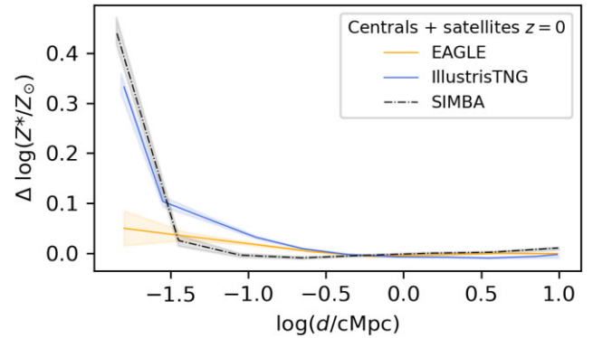
Figure 15. Distance from filaments dependence of the stellar metallicities' deviations from the MZR for all galaxies computed in EAGLE (orange line) and IllustrisTNG (blue line). The lines were obtained by binning the results in terms of distance and interpolating the corresponding medians. All the determinations are made for redshift z = 0 . Galaxies in all simulations are more metal-enriched (mainly satellites) in the filaments proximity, but IllustrisTNG and SIMBA show strong increases close to filaments, while EAGLE shows only a modest increase.
