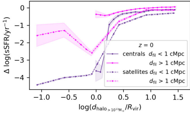
Figure 13. The deviations of the sSFR from the SFMS dependence on the distance to the closest massive halo ( M_h > 10^{13} M_\odot ) for centrals (continuous lines) and satellites (dashed lines), at redshift z = 0 . The galaxies outside filaments ( d > 1 cMpc) are considered separately, represented by the magenta lines. In addition to the halo effects, filamentary environments also play a non-negligible role in sSFR suppression.
