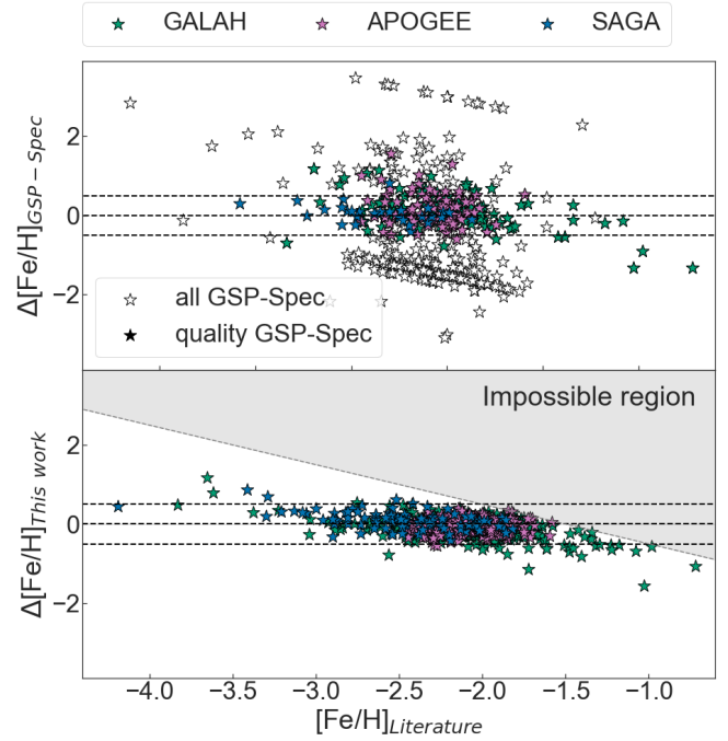
Fig. D.1. Precision of our metallicities (bottom) over GSP-Spec metallicities (top) validated using literature metallicities. The dashed lines shows the 0.0 \pm 0.5 dex metallicity difference lines. The gray shaded region in the bottom panel indicates the part of the figure where it's impossible to have data points due to the low metallicity selection ( [\text{Fe}/\text{H}]_{\text{This work}} < -1.5 ).
