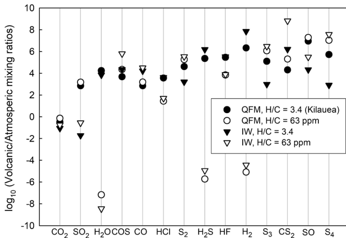
Fig. 2 Volcanic/Venus atmospheric gas ratios for Earth-like volcanic gases (filled symbols) and H-depleted gases (empty symbols). Concentrations of volcanic gases correspond to Kilauea-like compositions and H-depleted composition with the atmospheric H/C atomic ratio from Fig. 1. The atmospheric composition corresponds to observations ( \text{CO}_2 , \text{SO}_2 , \text{H}_2\text{O} , \text{CO} , \text{HCl} , \text{HF} ) and chemical equilibrium models for the near-surface atmosphere (Zolotov 1996). The figure demonstrates that most volcanic species before dilution and chemical interactions could be distinguished from atmospheric gases.
