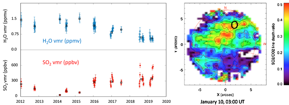
Fig. 7 Left: Long-term variations of the H 2 O volume mixing ratio (top, blue points) and the SO 2 volume mixing ratio (bottom, red points), measured at the cloud top from the TEXES data at 7.4 \mu m. From Encrenaz et al. (2020a, their Fig. 11); Right hand side panel: SO 2 :CO 2 line ratio map obtained by TEXES at 7.4 \mu m by Encrenaz et al. (2012), showing the large instantaneous spatial heterogeneity of SO 2 near cloud top.
