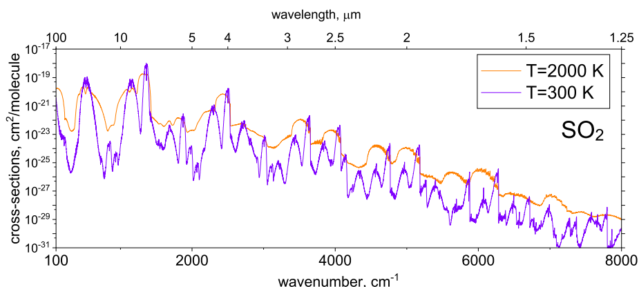
Figure 2. ExoMol Spectral Atlas (Tennyson & Yurchenko 2018): Cross-sections of \text{SO}_2 computed with the ExoMol line ExoAmes (Underwood et al. 2016).
