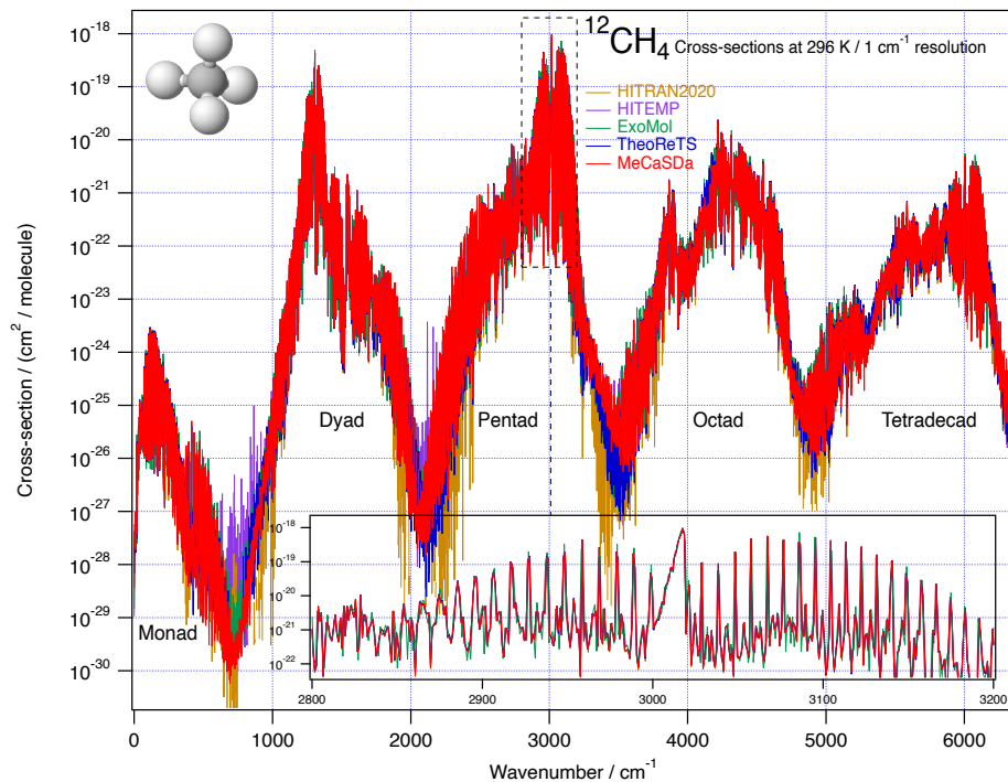
Figure 1. Comparison of ^{12}\text{CH}_4 cross-sections at 296 K in the far and mid-infrared regions for different databases: MeCaSDa (Ba et al. 2013), TheoReTs (Rey et al. 2016b), the ExoMol MM line list (Yurchenko et al. 2024a), HITRAN2020 (Gordon et al. 2022) and HITEMP (Hargreaves et al. 2020).
