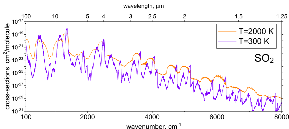
Figure 2. ExoMol Spectral Atlas (Tennyson & Yurchenko 2018): Cross-sections of SO 2 computed with the ExoMol line ExoAmes (Underwood et al. 2016).
