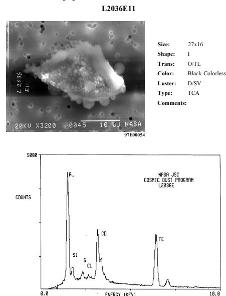
Figure 2: Typical Terrestrial Contaminant Artificial (TCA) particle from catalog 15 [6]
