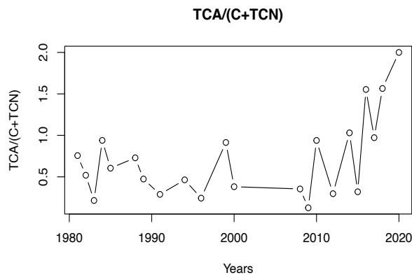
Figure 3: Ratio of the TCA to the C and TCN preliminary types of particles by year of collection published in the NASA Cosmic Dust Catalogs [4, 5]. A significant increase in the proportion of TCA particles can be noticed for the recent years.
