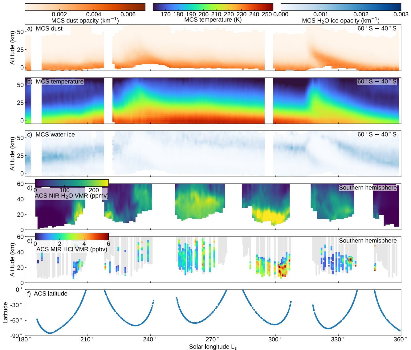
Figure 4. Example of the combined climatologies of dust, ice, temperature, H 2 O, and HCl. For the southern hemisphere in MY 35, shown are: (a) the dust opacity from MCS, (b) temperatures from MCS, (c) water ice opacity from MCS, (d) water vapor VMR from ACS NIR, and (e) HCl VMR from ACS MIR. Panel (f) shows the ACS solar occultation latitudes as shown in Figure 1 and Figure S4 in Supporting Information S1. The MCS data shown are zonally averaged using measurements from a mid-latitude band covering 60°S to 40°S. All altitudes are relative to the Mars areoid. Gray shading indicates periods and altitudes where secondary grating positions 11 and 12 were used, but the VMR of HCl was below the detection threshold.
