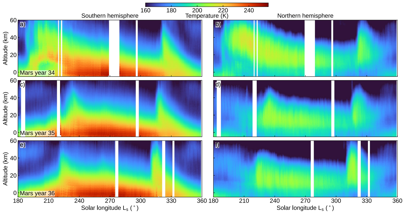
Figure 6. Climatology of temperature measured with MCS. Shown are vertical profiles of temperature measured with MCS as a function of L_s . MCS data are zonally averaged over latitude bands of 40^\circ\text{N} to 60^\circ\text{N} for the northern hemisphere, and 60^\circ\text{S} to 40^\circ\text{S} for the southern hemisphere. Panel arrangements by Mars year and hemisphere are as in Figure 3. Temperature measurements made using ACS NIR for the corresponding periods are shown in Figure S13 in Supporting Information S1.
