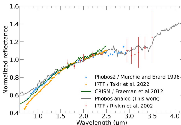
Figure 4: Comparison between the Phobos analog developed in this work and past observations of Phobos (red unit). The analog is a mixture composed of 60 vol.% of olivine, 20 vol.% of anthracite, and 20 vol.% of DECS-19. Our analog is in good agreement with the spectral slope in both visible and near-infrared.
