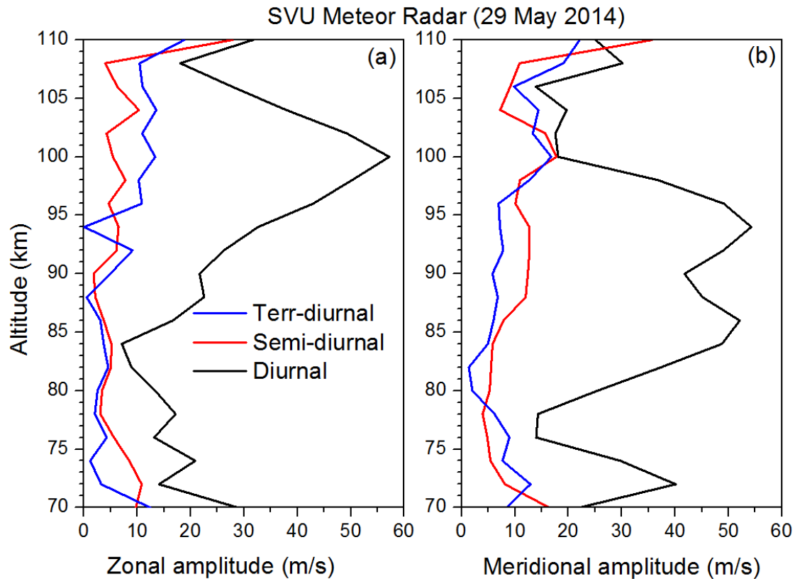
Figure 3. Profiles of diurnal, semi-diurnal and terr-diurnal tidal amplitudes observed in the (a) zonal and (b) meridional components obtained using S.V.U meteor radar on 29 May 2014. Here we can compared with Maura Hagan model output.
