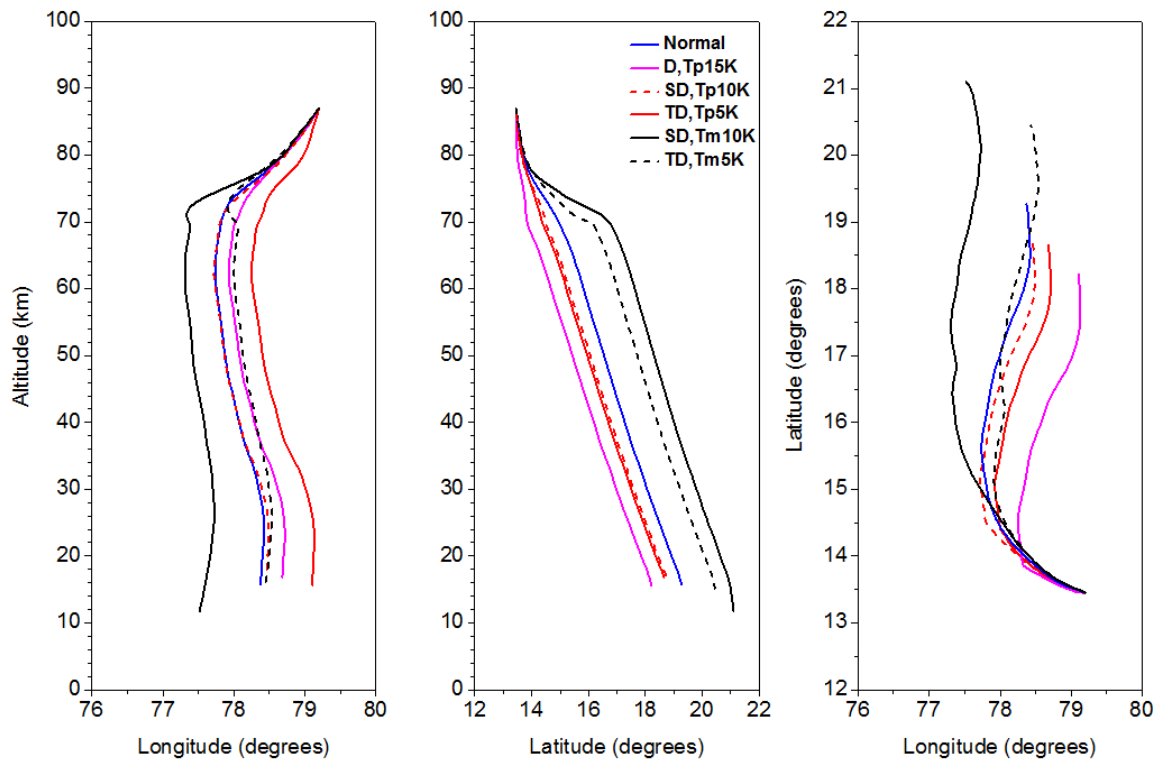
Figure 4. (a) Altitude vs. longitude, (b) Altitude Vs. latitude and (c) latitude vs. longitude variation of the ray paths obtained for the one of waves observed on 29 May 2014 using different background conditions. Blue line shows the actual wind and temperature data path of the wave. Ray paths obtained while using the observed diurnal (D), semi-diurnal (SD) and ter-diurnal (TD) amplitudes are also superimposed in the respective panels. Ray paths obtained while adding (p, red lines) or subtracting (m, black lines) the tidal amplitudes are also shown.
