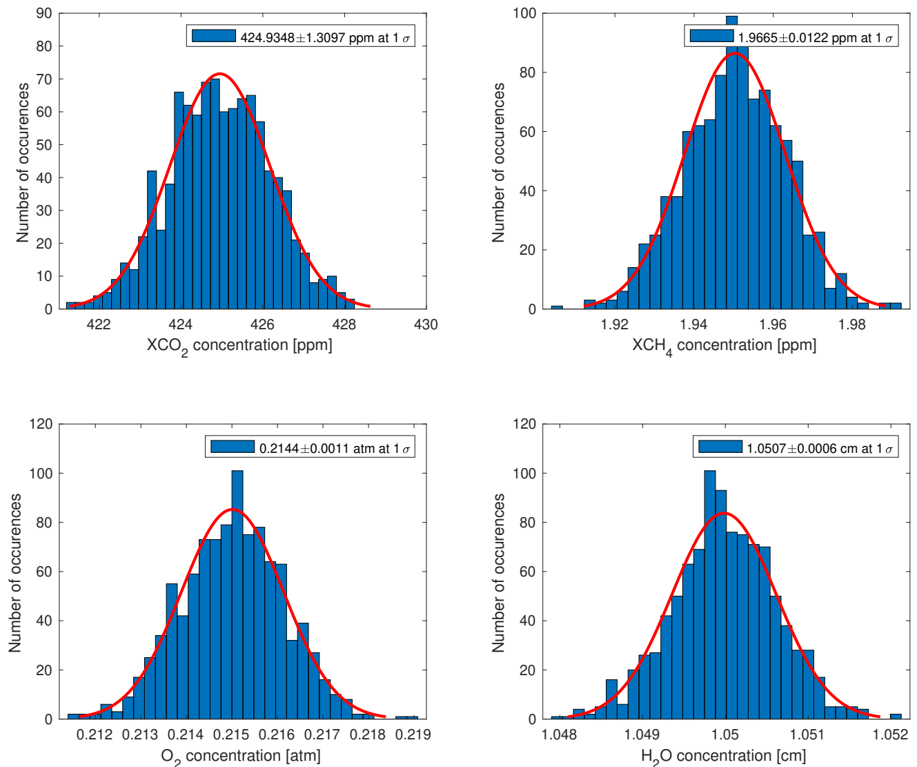
Figure 8. Retrieval of the concentration of gases that could be observed via the Uvsq-Sat NG NIR spectrometer (spectral resolution of 5 nm and SNR dependent on wavelength) for a specific observation scenario (targeted ‘Surface’—pine forest, ‘Aerosols’—continental, SZA of 20°). For obtaining the histograms, we find a mean square deviation equal to the uncertainty determined by the Levenberg–Marquardt algorithm.
