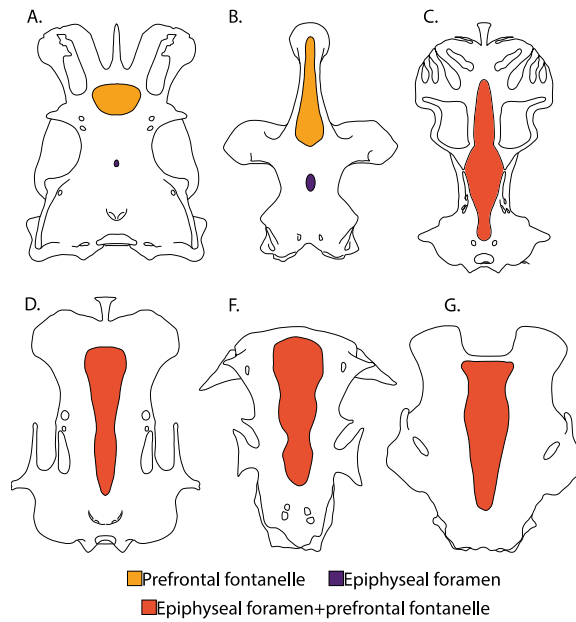
Figure S16. Line drawings of the character states recognized for character 26. A. Orectolobus ornatus (De Vis, 1883) (AMS 114236) (redrawn from Goto, 2001: text-fig. 9c). B. Trygonorrhina fasciata Müller and Henle, 1841 (MCZ 982S) (redrawn from McEachran et al. 1996: text-fig. 7). C. Parascyllium ferrugineum McCulloch, 1911 (HUMZ 131588) (redrawn from Goto, 2001: text-fig. 11c). D. Ginglymostoma cirratum (Bonnaterre, 1788) (ZMUC P0629) F. Gymnura japonica (Temminck and Schlegel, 1850) (HUMZ 4830) (redrawn from Nishida, 1990, text-fig 15A), G. Rhinoptera javanica Müller and Henle, 1841 (HUMZ 97698) (redrawn from Nishida, 1990, text-fig 17A). State [0]: A-B. State [1]: C-G.
