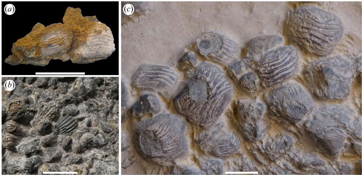
Figure S9. Tooth morphology of Ptychodus specimens MMSP CPC 3064, MMSP CPC 3065 and MMSP CPC 3068. (a) Two teeth extracted from specimen MMSP CPC 3064. (b) Portion of the dentition of specimen MUDE CPC 3065. (c) Portion of the dentition of specimen MMSP CPC 3068. Scale bars: 1 cm (b,c) and 5 mm (a).
