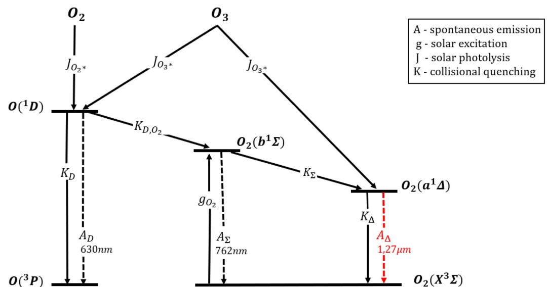
Figure 2. Illustration of the mechanisms resulting in the O_2(^1\Delta) dayglow at 1.27 \mu\text{m} (in red) implemented in the model. Adapted from Mlynarczyk et al. (1993).
