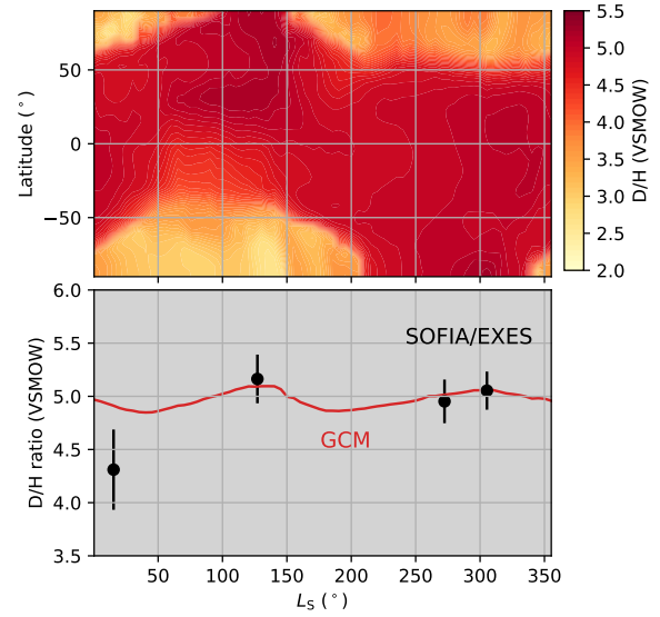
Figure 12. Annual cycle of the D/H ratio in the atmosphere of Mars. Simulations of the D/H ratio in water vapour in a GCM (and scaled by a factor of 1.05) suggest that it is subject to strong localised variations induced by the condensation of water vapour on the polar ice caps and ice clouds (top panel). On the other hand, the simulations suggest the planetary D/H ratio only varies up to 5% throughout a full Martian year (red line in bottom panel). The measurements of D/H from SOFIA/EXES (black dots in bottom panel) evidence the absence of strong variability in the global inventory of D/H, with the exception of the measurements made in L_S = 15^\circ , which depict a substantially lower value than the rest ( \sim 15\% ).
