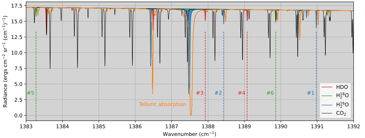
Figure 3. Modelled spectrum of the atmosphere of Mars at the spectral resolution of SOFIA/EXES. The coloured shadowed regions indicate the position and strength of the absorption lines of the water isotopes, while the black solid line indicates the absorption by \text{CO}_2 . The vertical dashed lines show the position of the absorption lines of each isotopologue considered in this study.
