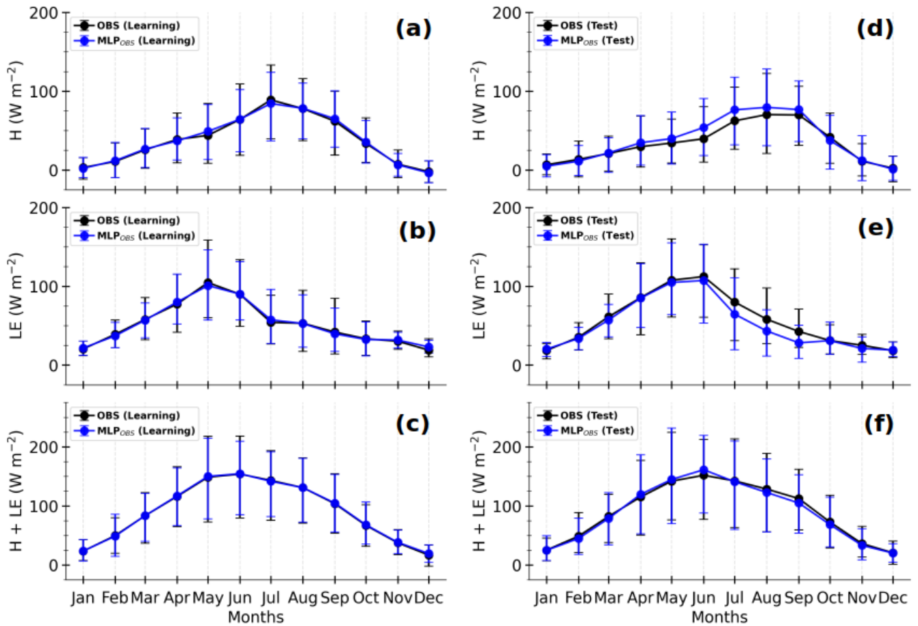
Figure 8. Composite monthly averages of observed and ( OBS in black) and MLP-based ( MLP_{OBS} in blue) sensible heat flux ( H , a and d), latent heat flux ( LE , b and e) and total turbulent heat flux ( H + LE , c and f) for the learning and test sets (left and right panels, respectively). The solid lines represent the means and the error bars correspond to 10 and 90 th percentiles, calculated by gathering the daily averages of half-hourly samples in Figure 6.
