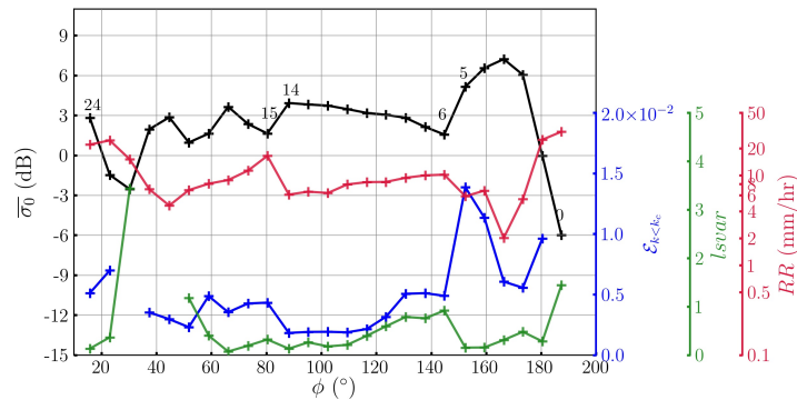
Figure 12: Values of \bar{\sigma}_0 (black), RR (red), l_{svar} parameter (green) and \mathcal{E}_{k>k_c} (blue) as a function of the azimuth direction, corresponding to the 25 footprints of the 10^\circ beam in box 78-1 (see Figure 20).
