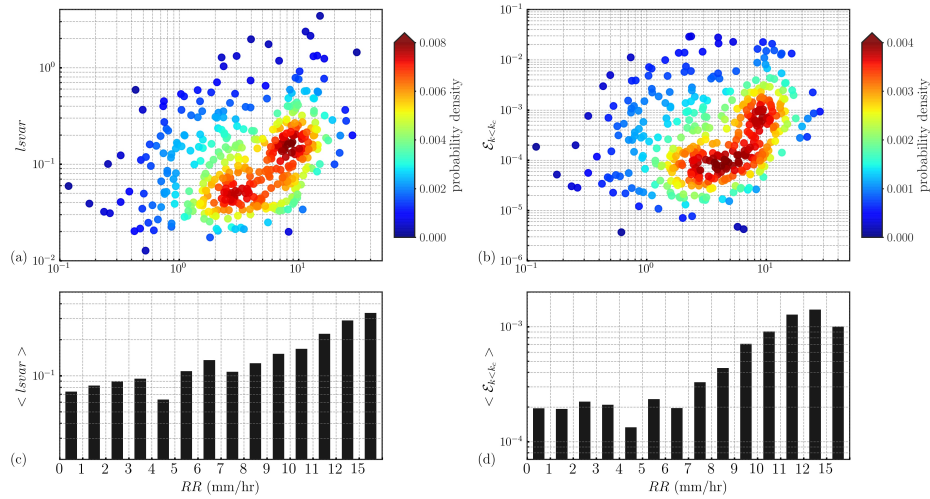
Figure 19: Scatterplot and probability density function (colors) of (a) the large-scale variability within the footprints ( lsvar ) and of (b) the energy \mathcal{E}_{k < k_c} , as a function of the rain rate RR at the middle of the 407 footprints of the 10^\circ spectral beam. Corresponding averaged values of (c) lsvar and of (d) \mathcal{E}_{k < k_c} per category of RR .
