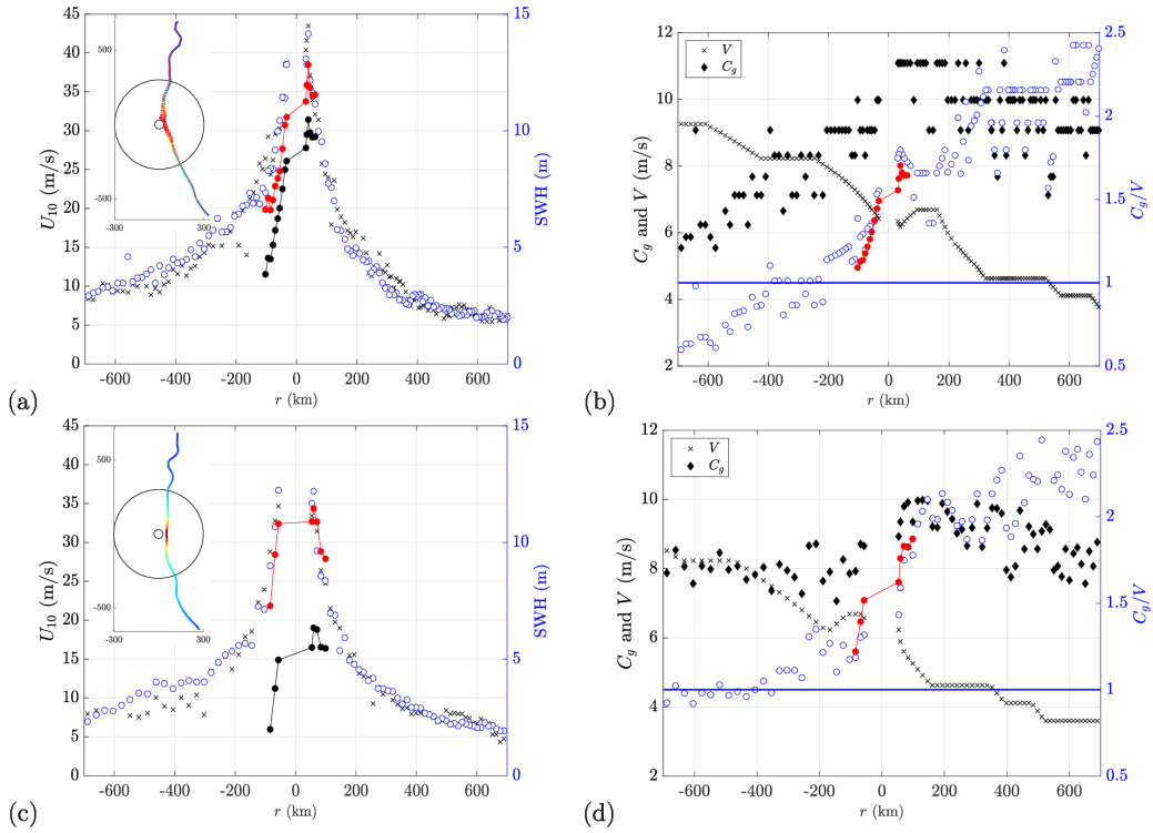
Figure 15: (a) Surface wind speed U_{10} (black crosses) and SWH measured by the SD (blue circles), superimposed to the SWH estimated by the KGC15 model using the translation velocity of SAM V (red line) or setting V = 0 m·s -1 (black line). (b) Group velocity C_g measured by the SD (black diamonds) and V (black crosses), superimposed to C_g/V (blue circles) and to its estimation by the KGC15 model (red line). Blue line indicates C_g/V = 1 . (c) and (d): Same as (a) and (b) but for the buoy 41044. Abscissa: distance to the TC center (defined with the same sign as y ). The trajectory in the frame of SAM of the SD and of the buoy 41044 (colored by the SWH and superimposed to the wind vectors) are shown on the insets in panels (a) and (c).
