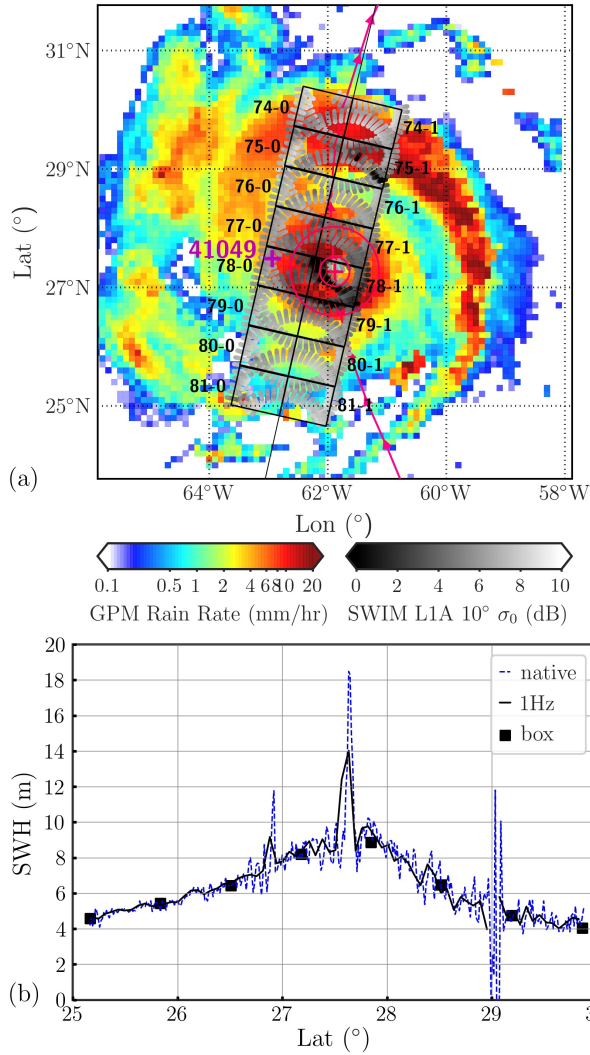
Figure 2: (a) SWIM footprints of the spectral beam at 10° during the passage of SWIM within SAM on 1st October 11:32. Gray color: values of \sigma_0 (in dB) along the footprints. In black: boxes of the L2 wave products, each side of the nadir track. In colors: rain field (mm/hr) on 1st October 11:30. Red line: trajectory of the center of SAM. Red cross: location of the center of SAM during the passage of SWIM. Red circles: R_{max} and 3R_{max} . Magenta cross: location of buoy 41049. (b) SWH as measured by SWIM along the nadir track: native (dashed blue), 1 Hz averaged (black) and averaged over each box (black squares).
