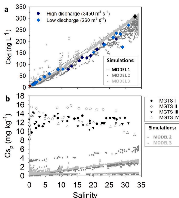
Fig. 8. Model output showing cation-exchangeable (a) Cs d and (b) Cs p reactivity for the simulated conditions (Model 1–3). In both cases, field Cs d and total particulate Cs p (presented in Figs. 4 and 5 for sampled points between Bdx_0 km and C_110 km) are overlaid for comparison. As a reminder: Model 1 simulates the conservative behavior, Model 2 Cs reactivity via cation-exchange on fresh SPM, and Model 3 Cs reactivity via cation-exchange on old SPM.
