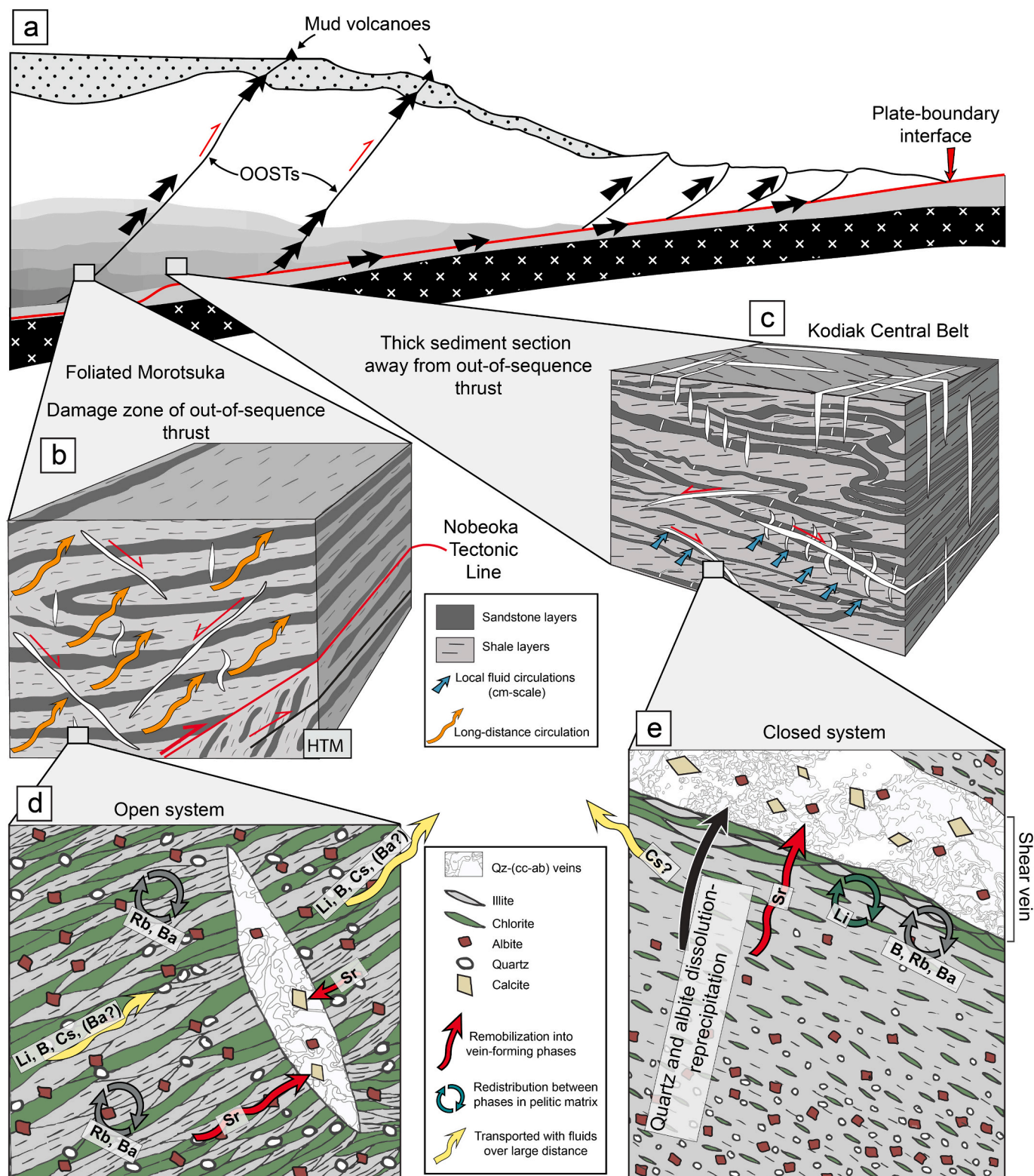
Fig. 14. The schematic scenario of FME budget evolution at studied sites, from the location within the wedge down to thin section: (a) A sketch of an accretionary wedge redrawn after Kastner et al. (2014) with the relative locations of studied units, the Foliated Morotsuka and the Kodiak Central Belt. The Foliated Morotsuka is located in the hanging wall of the out-of-sequence thrust (Nobeoka Tectonic Line), whereas the Kodiak Central Belt was underplated in the middle of thick turbiditic sequence far from any large-scale faults. A 3D sketch of (b) the Foliated Morotsuka and (c) the Kodiak Central Belt with presented deformation structures and possible scenarios for fluid flow. (d) and (e) show details of the mineralogy of metapelites from both localities and their influence on FME budget. In the Foliated Morotsuka (d), Li, B, Cs, and \pm Ba are leached from the host rock, with only Sr stored in vein-forming calcite. Conversely, in the Kodiak Central Belt (e), Li, B, Rb, and Ba are reorganized between illite, chlorite and albite and Sr being stored in the vein calcite. Only a small proportion of Cs is potentially lost to the fluid.
