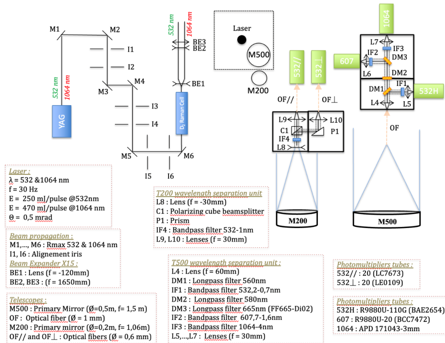
Figure 3 : LiO3T optical scheme
