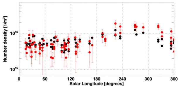
Fig. 4 Seasonal variation of the CO 2 density at 140 km (red dots). The black dots indicate the densities predicted by the MCD that were used as a priori values in the retrieval process. Reproduced with permission from Aoki et al. (2022), copyright by AGU
