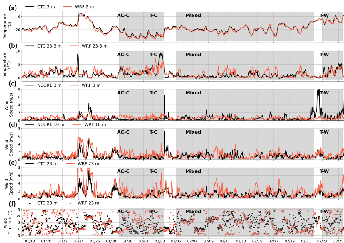
Figure B1. Time series of surface and near-surface temperatures (°C), temperature gradients (dT) (°C), wind speeds ( \text{ms}^{-1} ) and directions (deg.), at Downtown, compared to EPA-WRF (red) for available observations (black) up to 23 m altitude during ALPACA-2022.
