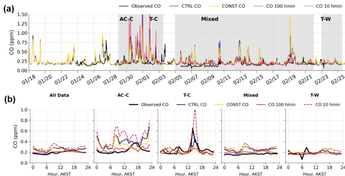
Figure E2. a) Total modelled surface and power plant tracers as a function of time between 0-5 m for CTRL and selected sensitivity simulations described in Table 2 compared to available surface observations, at UAF Farm for CO. b) Average diurnal cycles at UAF Farm for observations (black) and model simulations (colours as in (a)) for CO averaged over all data and for events A-C, T-C, Mixed and T-W.
