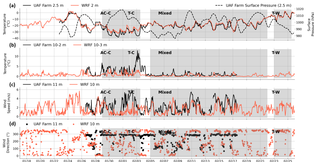
Figure B2. Time series of surface and near-surface temperatures ( ^{\circ}\text{C} ), temperature gradients ( dT ) ( ^{\circ}\text{C} ), wind speeds ( \text{ms}^{-1} ) and directions (deg.), at UAF Farm, compared to EPA-WRF (red) for available observations (black) up to 11 m altitude during ALPACA-2022.
