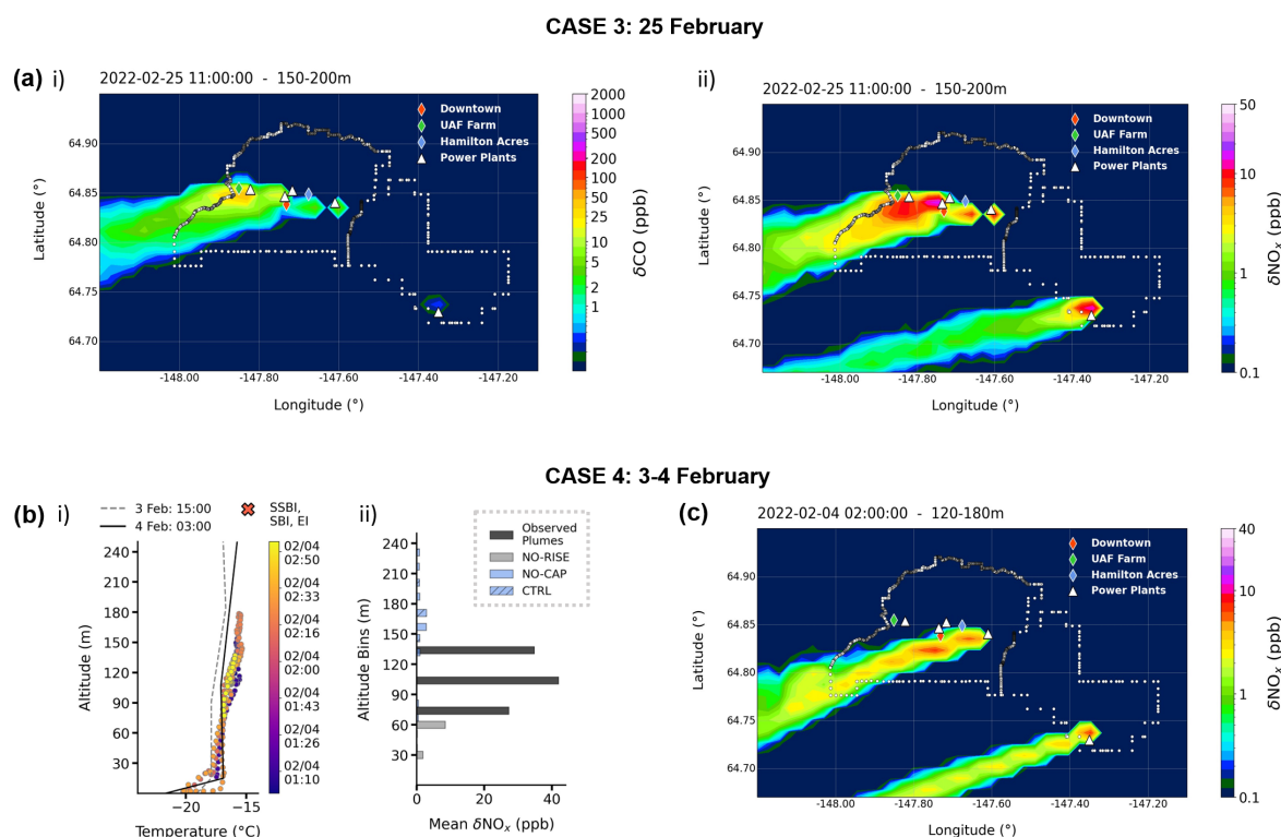
Figure D2. a) Spatial distribution of power plant tracers for i) CO (ppb) and ii) NO x (ppb) between 150-200 m at 1100 AKST on 25 February (Case 3, Section 5), highlighting the Aurora plume displacement to the south of the UAF Farm. b) Observed temperature profiles and modelled NO x tracer (ppb) enhancements against observations averaged over 30 m altitude bins for Case 4 on 3-4 February (see Fig. 7 for details). c) Spatial distribution of power plant NO x tracer (ppb) between (120 - 180 m) at 0200 AKST on 4 February, highlighting the Doyon plume displacement to the south of the UAF Farm.
