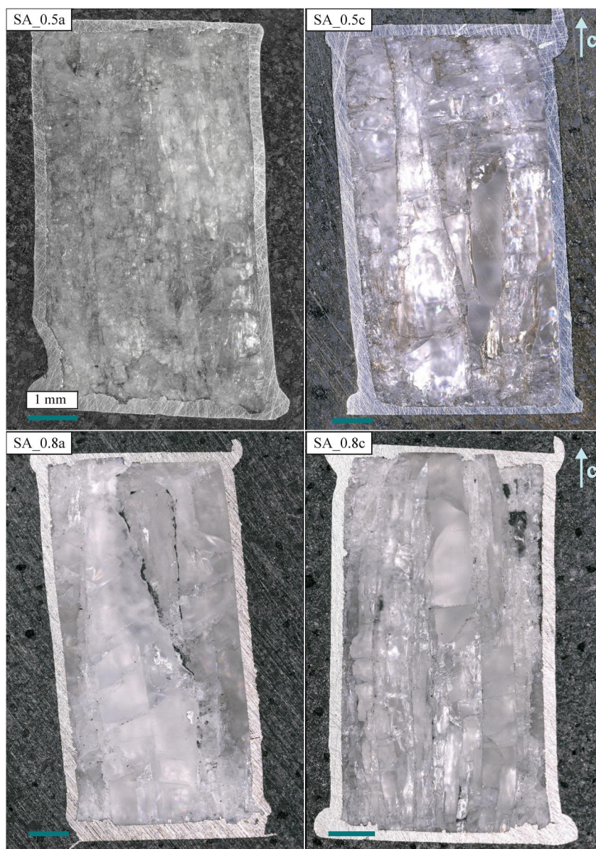
Figure 7. Images of quartz single-crystal samples from experiments at 0.5 and 0.8 GPa. Two samples were cored parallel to c -axis and the other two perpendicular to c -axis, as indicated in the top right corner of each image. Scale bar is 1 mm long on all images. The vertical and horizontal cracks are not present in the samples prior to the experiment; their origin is discussed in Section 3.3.
