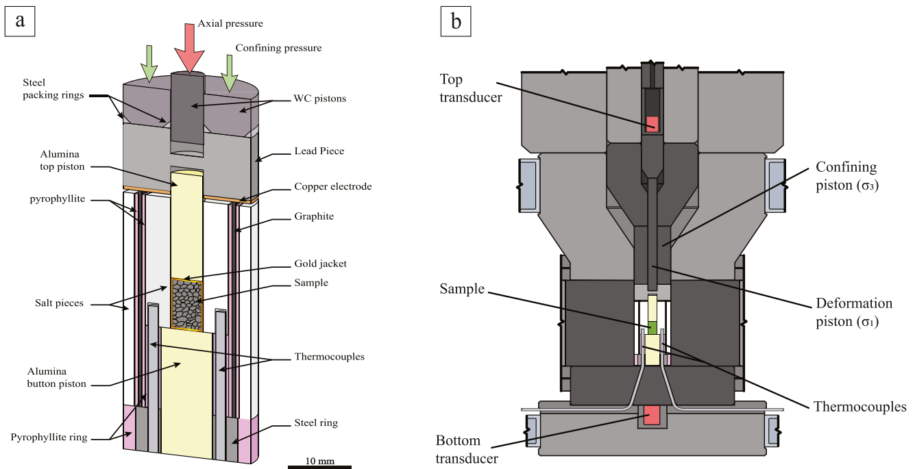
Figure 1. (a) Vertical cross-section of the sample assembly. (b) Schematics of the Griggs set-up with the position of the sample assembly and of the ultrasonic transducers.
