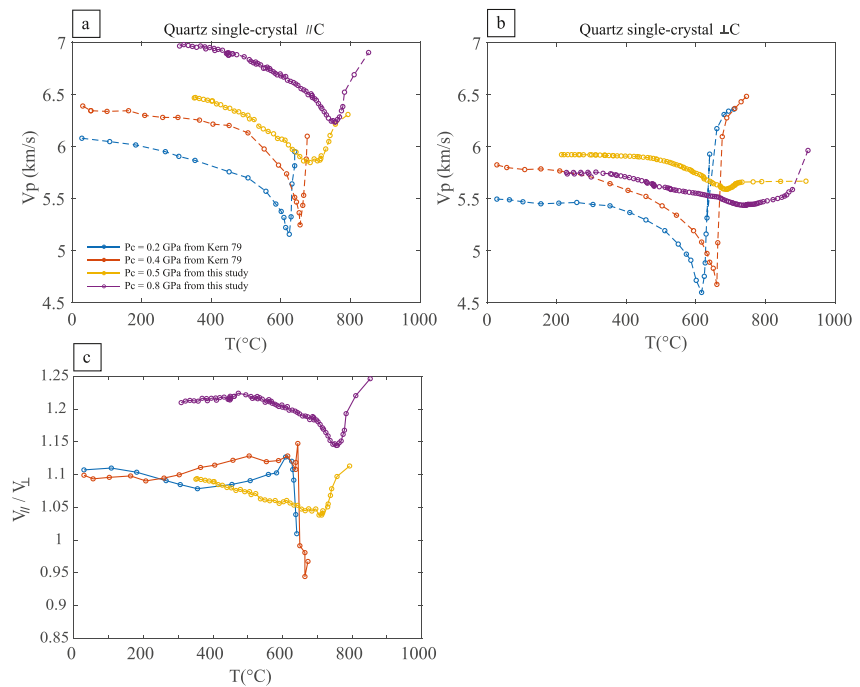
Figure 11. P-wave velocity in quartz single crystals versus temperature (a) V_{\parallel c} along the c -axis, (b) V_{\perp c} along the a -axis, and (c) P-wave anisotropy V_{\parallel}/V_{\perp} . The yellow and purple curves represent data obtained at 0.5 and 0.8 GPa, respectively. The blue and red curves represent experimental data from Kern (1979) at 0.2 and 0.4 GPa, respectively.
