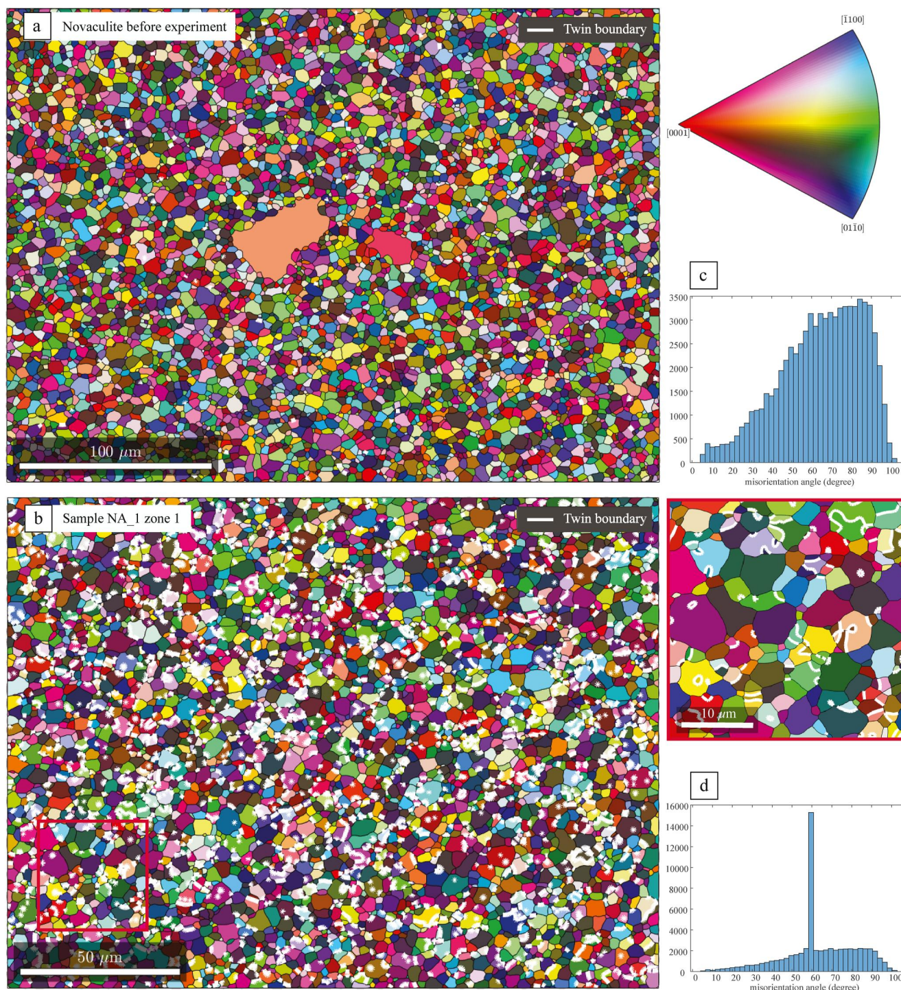
Figure 9. Electron Back Scatter Diffraction (EBSD) image of (a) the novaculite starting material and (b) sample of experiment NA_1 at 1 GPa. White lines represent Dauphiné twin boundaries. Panels (c) and (d) are histograms of novaculite grain misorientations for maps shown in (a) and (b), respectively. The red rectangle on the right shows a magnified view according to the rectangle in (b).
