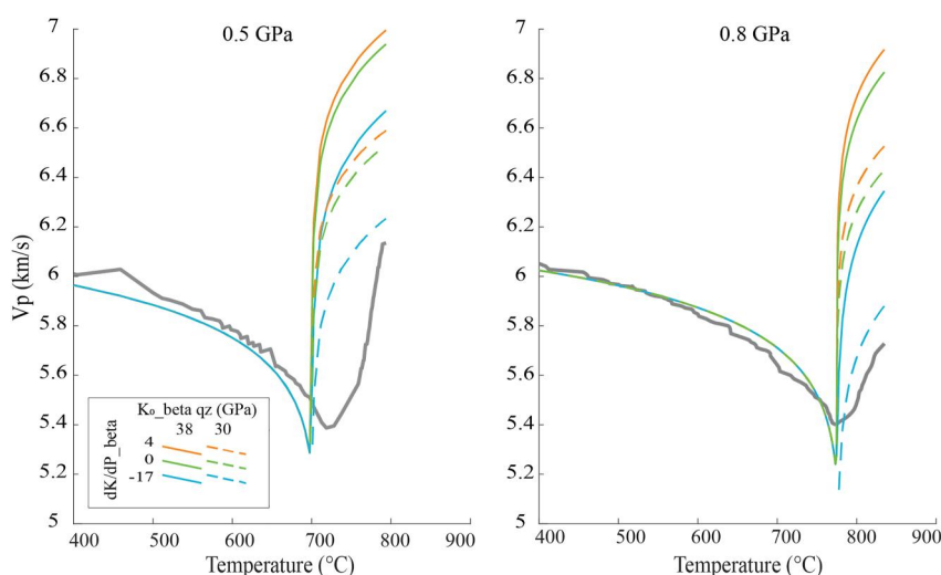
Figure 14. P-wave velocity versus temperature for different values of K_o and K' ( =dK/dP ) for \beta quartz. Left, 0.5 GPa; right, 0.8 GPa. Gray solid lines represent data points obtained in this study. Solid and dashed lines are calculations with room pressure bulk moduli of K_o = 38 GPa and K_o = 30 GPa, respectively. Orange, green and blue curves represent calculations for K' equal to 4, 0, and -17 respectively.
