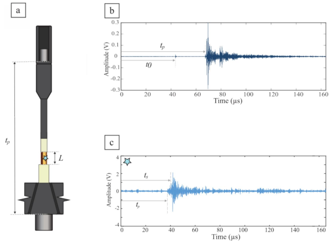
Figure 2. (a) Acoustic monitoring set-up. t_p is the travel time between the two transducers and L the sample length (b) Typical waveform recorded by the top transducer during a velocity survey. t_o is the time at which the pulse is sent to the bottom transducer. (c) Typical waveform of an acoustic emission generated inside the sample and recorded by bottom transducer, amplified at 60 dB and high-pass filtered above 500 KHz.
