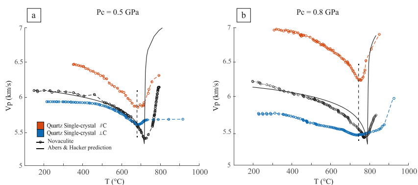
Figure 6. P wave velocities in novaculite versus quartz single crystal. Black solid lines represent the prediction of Abers and Hacker (2016), black circles are the present data obtained on Novaculite, red and blue circles are from single crystal c -axis-parallel and -perpendicular measurements, respectively. (a) 0.5 GPa (experiments SA_{0.5a} and SA_{0.5c} ) and (b) 0.8 GPa (experiments SA_{0.8a} and SA_{0.8c} ).
