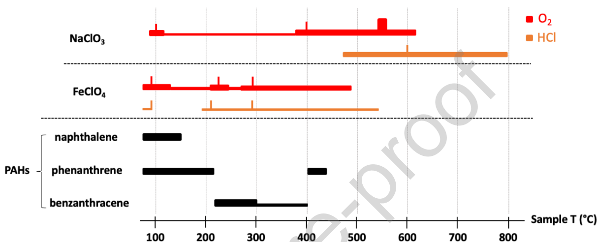
Figure 6. Summary of the release temperatures of the volatiles O 2 and HCl for NaClO 3 and FeClO 4 which were the most impactful oxychlorines of all the salts targeted compared to the release temperatures of the three PAHs selected for this study. The release temperatures of all volatiles for all six salts can be found in the supplemental Figure S1.
