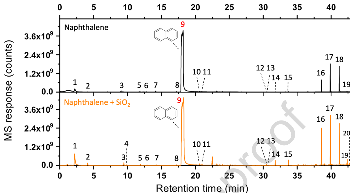
Figure 2. Chromatograms obtained after the pyrolysis of ~0.15 mg of pure naphthalene (black) compared to 0.5 wt% of naphthalene mixed in fused silica (orange). The highest abundance compounds that were detected correspond to: 1. CO 2 , 2. benzene, 3. phenylethyne, 4. styrene, 8. methylene-indene, 9. naphthalene (parent molecule), 10. 2-methylnaphthalene, 11. 1-methylnaphthalene, 12. phenanthrene, 13. anthracene, 14. vinylanthracene, 15. phenylnaphthalene, 16. triphenylene, 17. 1,1-binaphthalene, 18. 1,2-binaphthalene, 19. benzofluoranthene, and 20. dinaphthofurane.
