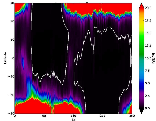
Figure 1: Zonal mean peak limb NO emission at LT=21 predicted by the LMD-MGCM
