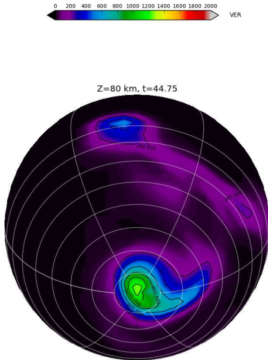
Figure 2: GCM simulation of the NO volume emission rate at an altitude of 80 km at L_s=0 , around the South pole of Mars
