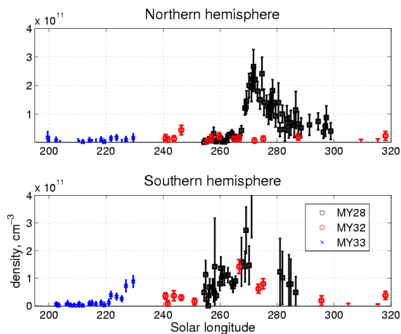
Figure 4. H 2 O density in MY28, 32, 33 at 60 km.
