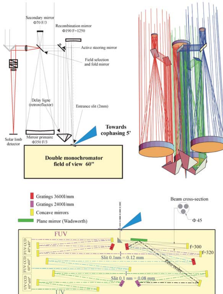
Figure 1 SOLARNET Design.
