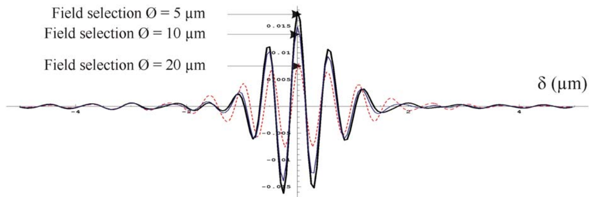
Figure 3 Fringes pattern for an high resolution white source and a spatial filter.
