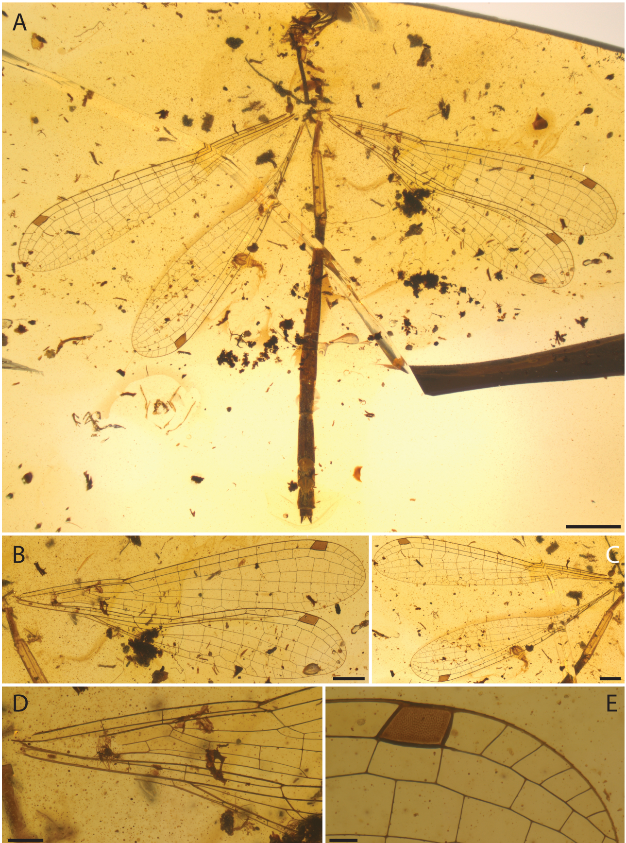
FIGURE 1. Mesosticta additicta sp. nov., holotype NIGP204970. A , Habitus in dorsal view. B , Right wings. C , Left wings. D , Detailed view of bases of right wings. E , Detailed view of pterostigma. Scale bars = 2 mm (A), 1 mm (B, C), 0.5 mm (D), 0.2 mm (E).
