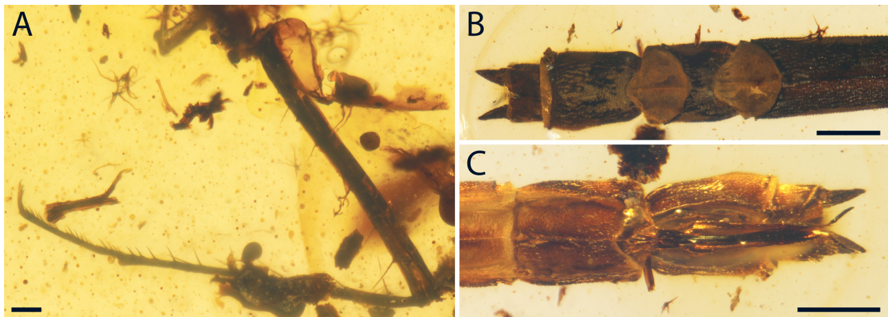
FIGURE 2. Mesosticta additicta sp. nov., holotype NIGP204970. A , Detailed view of hind leg. B , Dorsal view of abdomen apex. C , Ventral view of abdomen apex. Scale bars = 0.2 mm (A), 0.5 mm (B, C).
