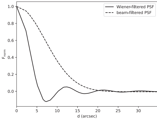
Figure 2. The effective Point Spread Function (PSF) profile in a PPI1 image after applying a Wiener filter (solid line) or a naïve PSF filter (dashed line). The naïve filter is optimal for flux estimation of isolated point sources, including non-local data with reduced weight, to enhance the signal-to-instrumental noise ratio in comparison to a central, purely local estimate. The Wiener filter has a much narrower central beam, which provides some reduction in instrumental noise but is balanced against adding confusion noise from non-local data. The Wiener filter also has a negative feature (at around 7 arcsec in this example), which provides a local background subtraction, actively reducing confusion noise.
