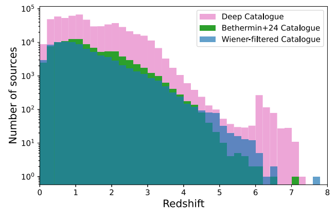
Figure 3. Redshift distribution for the three prior source catalogues considered in Section 4.2: The Deep catalogue (pink) of \sim 590\,000 sources which all have a flux greater than 1 \mu\text{Jy} in the PH11.1 channel, the catalogue of blindly detected sources in the noiseless maps (green) from B24 of \sim 102\,000 sources and the catalogue of blindly detected sources in the Wiener-filtered, noisy maps (blue) with \sim 83\,000 sources.
