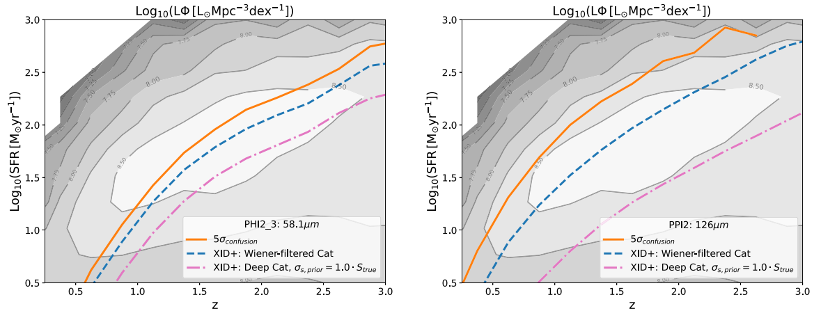
Figure 8. Regions of the redshift–SFR plane accessible to PRIMAger at the given limiting fluxes reached by XID+ in the PH12.3 (left) and PPI2 (right) channels. Sources that lie within above the lines are those whose fluxes can be accurately measured in the given channels using XID+. Additionally, the FIR luminosity density as a function of redshift and SFR is shown by the grey-scale contours. The classical confusion limits from B24 in each channel are shown by the solid orange lines. The limiting fluxes from XID+ with the Wiener-filtered prior catalogue and the Deep prior catalogue with flux priors of \sigma_{s,\text{prior}} = S_{\text{true}} are shown by the blue-dashed lines and the dash-dotted pink lines, respectively.
