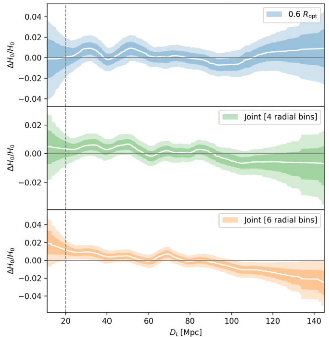
Figure 8. Top: We show the 1\sigma and 2\sigma C.L. of the fit to the 0.6 R_{\text{opt}} bin. Centre: Similar to the top panel, for the baseline joint analysis with the four radial bins and for comparison, we also show the results from all the six radial bins in the Bottom panel.
