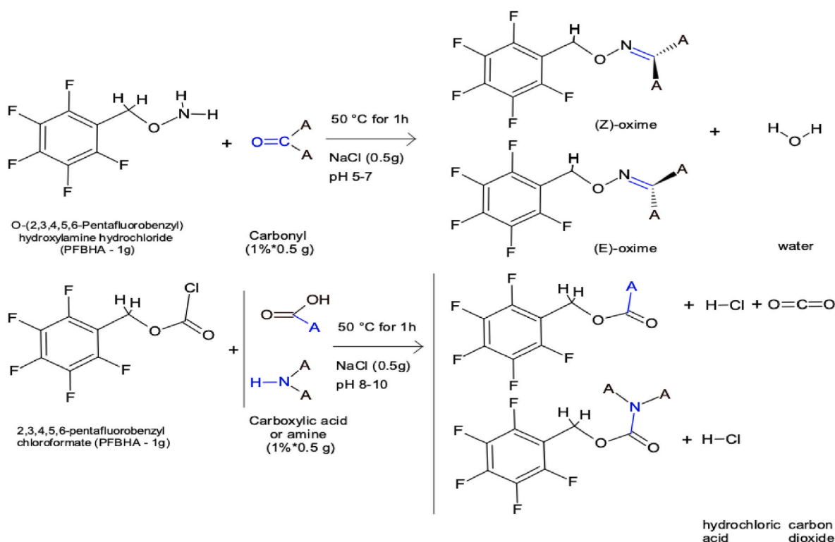
Fig. 4. SPME PFBHA and PFBCH reactions and GC-MS analysis results with the list of compounds identified and specified for the one derivatized.
