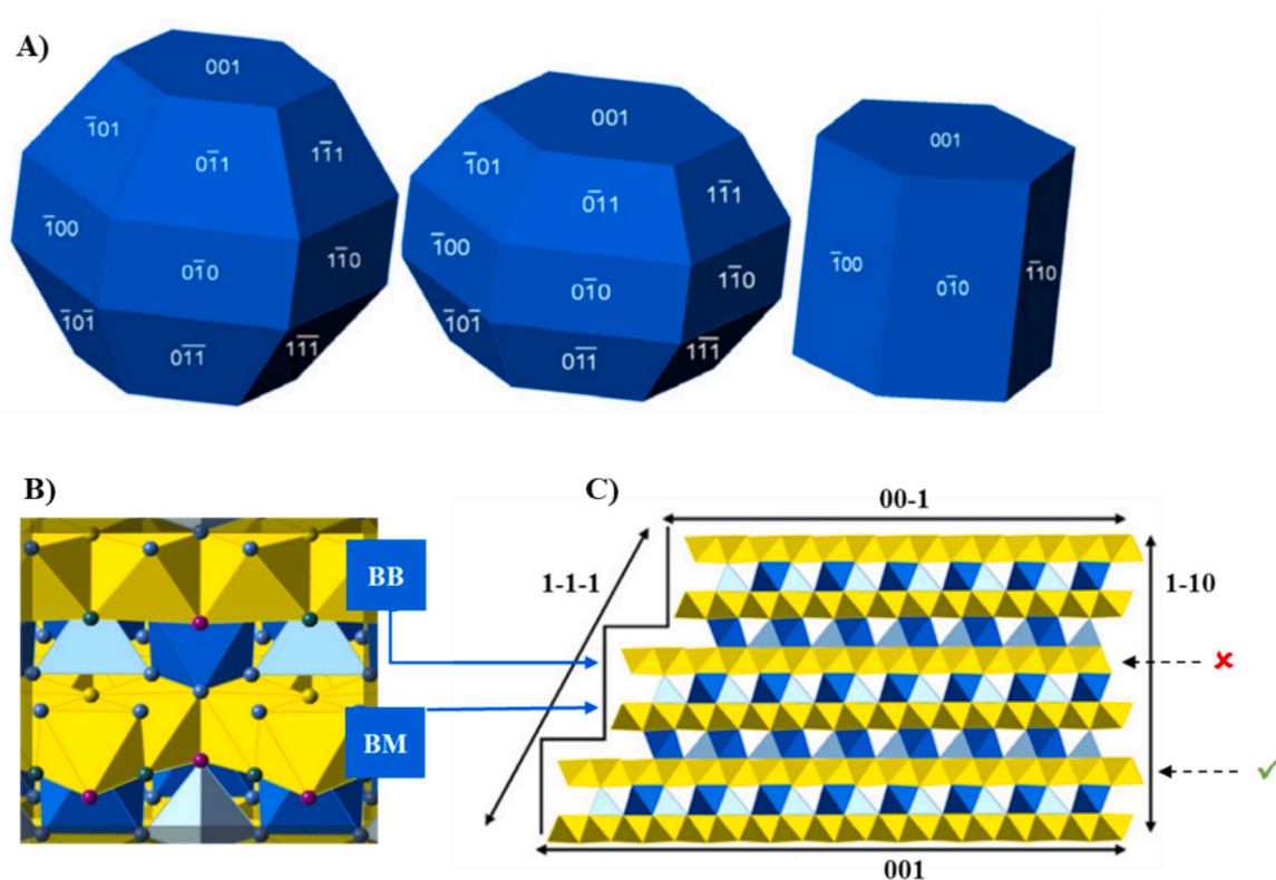
Fig. 9. Idealized ferrihydrite shape figure adjusted from Fig. 7 in Hiemstra et al., 2013. A) idealized Fh shapes and their respective surfaces, B) sorption site morphology, and C) crystal terminations as found on each type of plane. With the difference in BM complex sorption site variation on the (1-10) plane indicated by the dashed arrows, the tick mark indicating an available sorption site and the cross an unavailable adsorption site.
